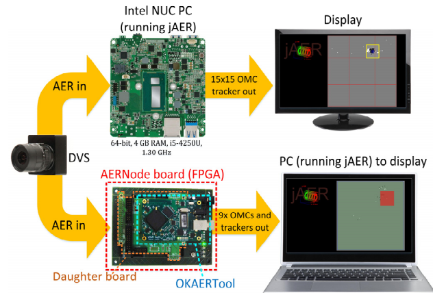
Fig. 1 Illustration of the two possible AER processing pathways of the demonstration: software-based (top) and FPGA-based (bottom).
