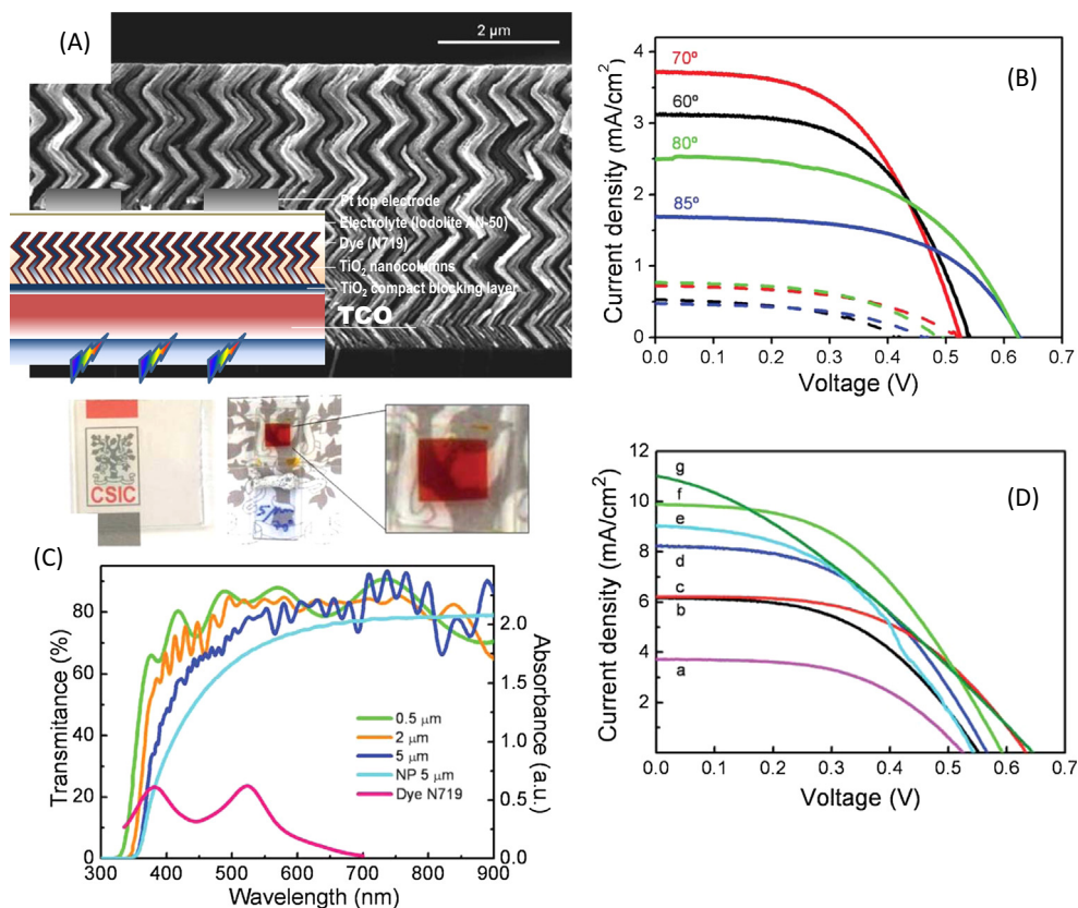
Fig. 5.6. TiO 2 as DSSC photoanode. (A) Cross-sectional SEM micrograph of a zigzag thin film consisting of ten stacked 500 nm TiO 2 layers (5 μm total thickness) prepared by successive azimuthal rotation of the substrate by 180°. The inset shows a schematic of the DSSC device. (B) I - V curves for TiO 2 photoanodes deposited at different angles and used either as prepared (dashed lines) or after crystallization by annealing at 400 °C (full lines). (C) UV-vis transmission spectra for a series of OAD TiO 2 films with different thicknesses consisting of single and stacked 500 nm-thick layers prepared in a zigzag configuration. The transmission spectrum of a nanoparticle thin film and the absorption spectrum of the N719 dye solution are included for comparison. The photographs presented in the top of the panel correspond to a 5 μm-thick zigzag film infiltrated with dye to show the high transparency of the final cells. (D) I - V curves obtained from DSSCs utilizing zigzag TiO 2 thin films grown at \alpha \approx 70^\circ to thicknesses of: (a) 500 nm, (b) 1 μm, (c) 1.5 μm, (d) 2 μm, (e) 2.5 μm, (f) 3 μm and (g) 5 μm [63].
