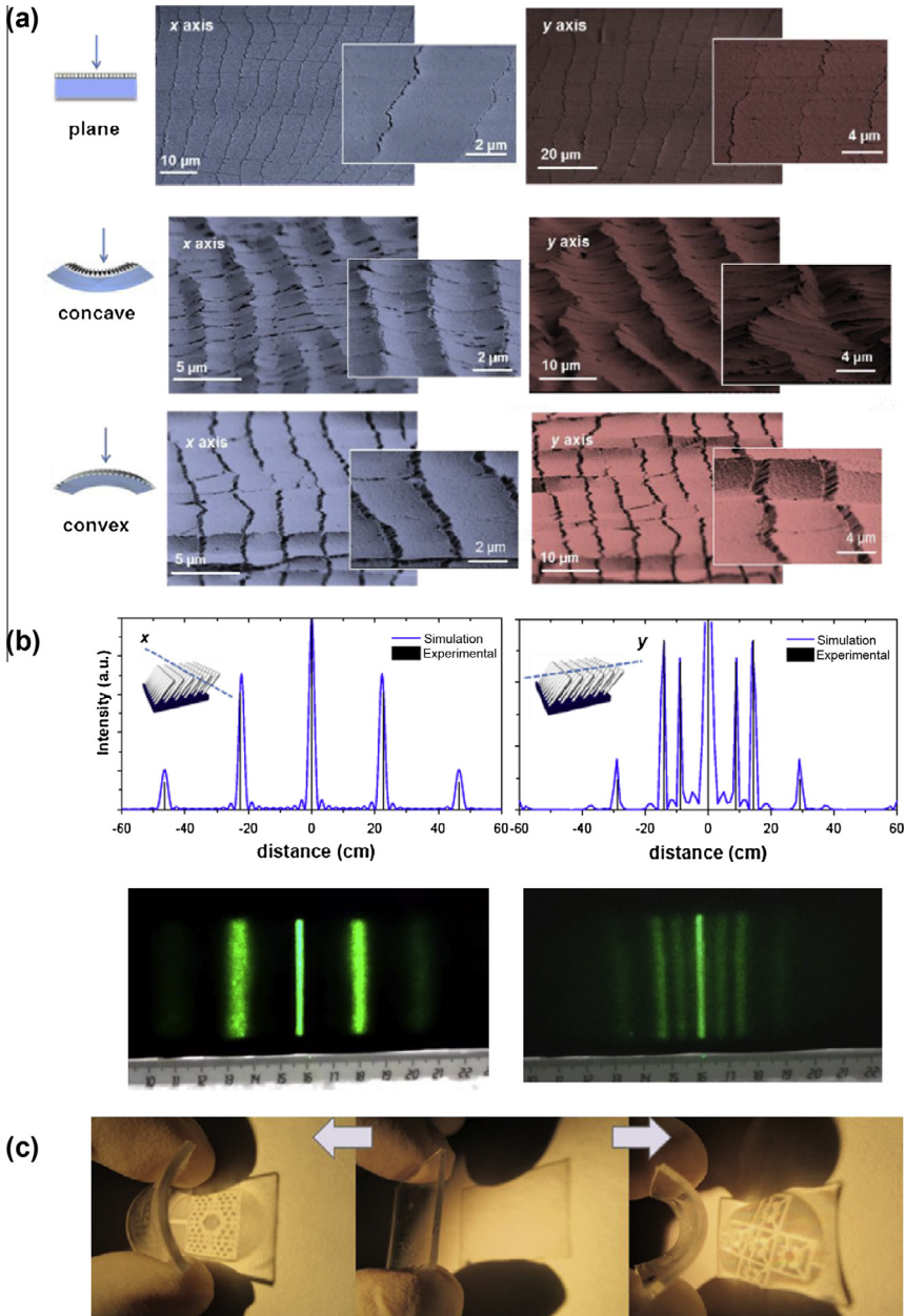
Fig. 5.12. (a) SEM micrographs of two PDMS foils coated with nanocolumnar \text{SiO}_2 films deposited by OAD. The images correspond to a flat foil (top) and to the same foil bent to form a concave (middle) or convex (bottom) surface, as indicated. The foils were bent along the film's bundling x -axis (left panel in blue) and along its growth y -axis (right panel in red). (b) Fraunhofer diffraction patterns obtained by illuminating a concave surface bent along the bundling x - (right) and growth y - (left) axes with a 532 nm laser beam. The experimental diffraction patterns can be simulated by assuming a Fraunhofer diffraction by the periodic undulation observed in the concave surfaces shown in (a). (c) Examples of invisible labels fabricated by depositing a nanocolumnar \text{SiO}_2 thin film on each side of a PDMS foil using two different shadow masks. The flat double-sided coated foil is transparent (central picture). The projected light reveals the pattern printed on the concave surface, whereas the pattern on the opposite convex surface remains invisible (left and right pictures) [507].
