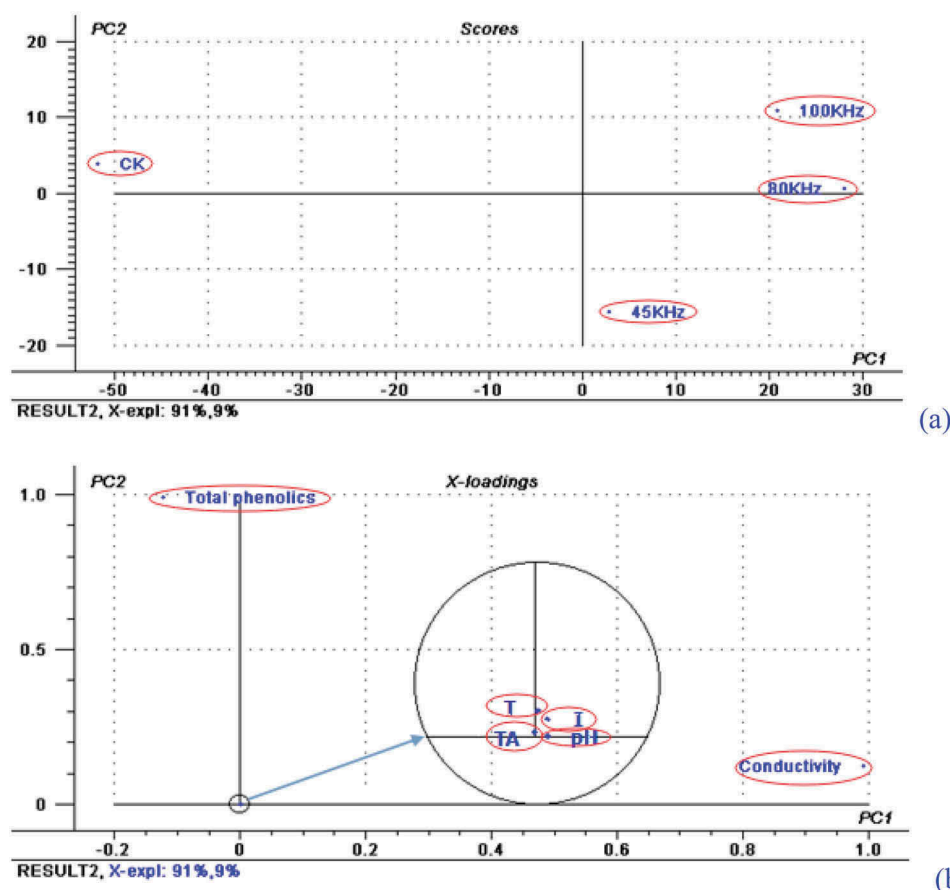
Figure 2. PCA scores (a) and loadings (b) for PC1 and PC2 of physicochemical properties of a red wine sonicated with different frequencies.
