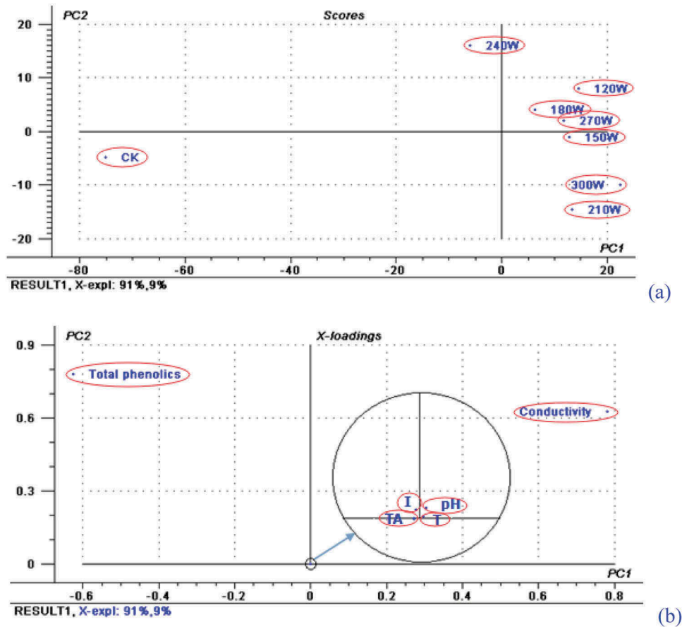
Figure 1. Scatterplot of scores (a) and loadings (b) for PCA1 and PC2 of samples treated at different ultrasonic power.
