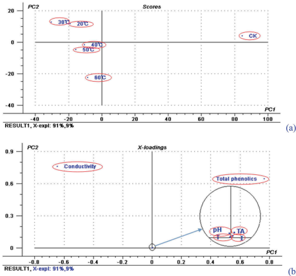
Figure 3. Scores plot (a) and loadings plot (b) for PC1 and PC2 of samples sonicated at different temperatures.
