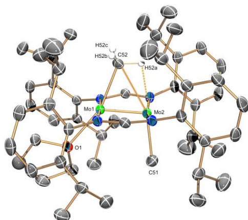
Figure 3. The solid state molecular structure of the tetrahydrofuran adduct [\text{Mo}_2\text{Me}(\mu\text{-Me})\{\mu\text{-HC}(\text{NDipp})_2\}_2(\text{THF})] . Solid-state molecular structure of complex 3-THF with thermal ellipsoids set at 50% probability. Some hydrogen atoms have been omitted for clarity. Selected bond lengths (Å) and angles ( ^\circ ): Mo(1)–Mo(2), 2.086(1); Mo(1)–O(1), 2.258(2); Mo(1)–C(52), 2.220(3); Mo(2)–C(52), 2.573(3); Mo(2)–C(51), 2.214(3); C(52)–Mo(1)–O(1), 160.4(1); C(52)–Mo(2)–C(51), 156.7(1); Mo(1)–C(52)–Mo(2), 51.0(1); O(1)–Mo(1)–Mo(2), 126.3(1); Mo(1)–Mo(2)–C(51), 101.0(1).
