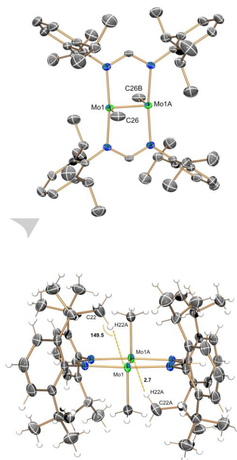
Figure 2. X-ray molecular structure of [Mo 2 Me 2 { \mu -HC(NDipp) 2 } 2 ] ( 2 ), emphasizing the coordinative unsaturation of the Mo atoms (above) and the possible existence of weak \epsilon -agostic interactions (bottom drawing). Anisotropic displacement parameters drawn at the 50% level. Selected bond lengths (Å) and angles (°): Mo(1)-Mo(1A), 2.080(1); Mo(1)-C(26), 2.189(3); Mo(1A)-Mo(1)-C(26), 92.8(1).
