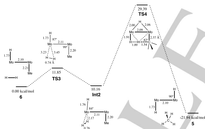
Scheme 6. Stationary points along subsequent hydrogenation reaction of 6 and their relative free energies. Some relevant bond distances and angles are also shown.
