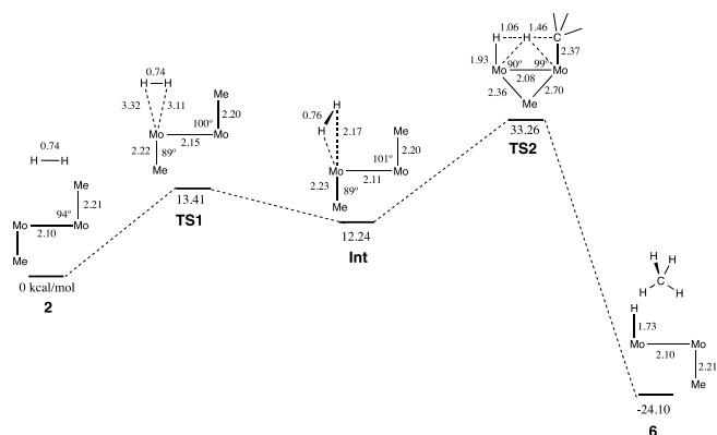
Scheme 5. Stationary points along hydrogenation reaction of 2 and their relative free energies. Some relevant bond distances and angles are also shown.
