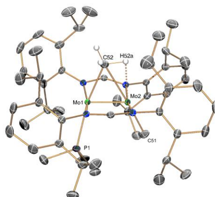
Figure 4. Solid-state molecular structures of complexes 3-PMe 3 with thermal ellipsoids set at 50% probability. Selected bond lengths (Å) and angles ( ^\circ ): Mo(1)–Mo(2), 2.088(1); Mo(1)–P(1), 2.591(1); Mo(1)–C(52), 2.292(2); Mo(2)–C(52), 2.492(2); Mo(2)–C(51), 2.192(2); C(52)–Mo(1)–P(1), 166.1(1); C(52)–Mo(2)–C(51), 175.5(1); Mo(1)–C(52)–Mo(2), 51.5(1); P(1)–Mo(1)–Mo(2), 102.3(1); Mo(1)–Mo(2)–C(51), 117.2(1).
