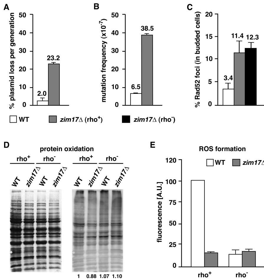
Figure 2. The zim17 \Delta mutants exhibit higher levels of plasmid loss, mutation frequency and Rad52-YFP foci and reduced levels of protein oxidation and respiration. (A) Plasmid loss as determined by the percentage of pRS315-retaining cells after overnight growth on non-selective medium. (B) Mutation frequencies were calculated by fluctuation tests of canavanine resistant colony formation. (C) Rad52-YFP foci formation in S/G2 phase of \rho^+ (gray bar) and \rho^- (black bar) strains. (D) Total amount of protein determined by Coomassie staining (left) and protein carbonylation (right). Quantification is indicated (bottom). (E) Intracellular ROS levels determined by dihydroethidium.
