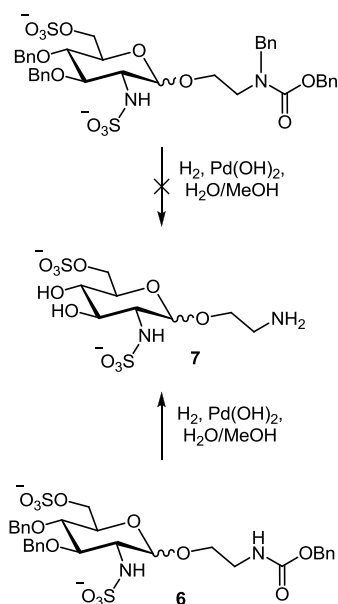
Scheme 2. Previous experiments with glucosamine monosaccharides.
