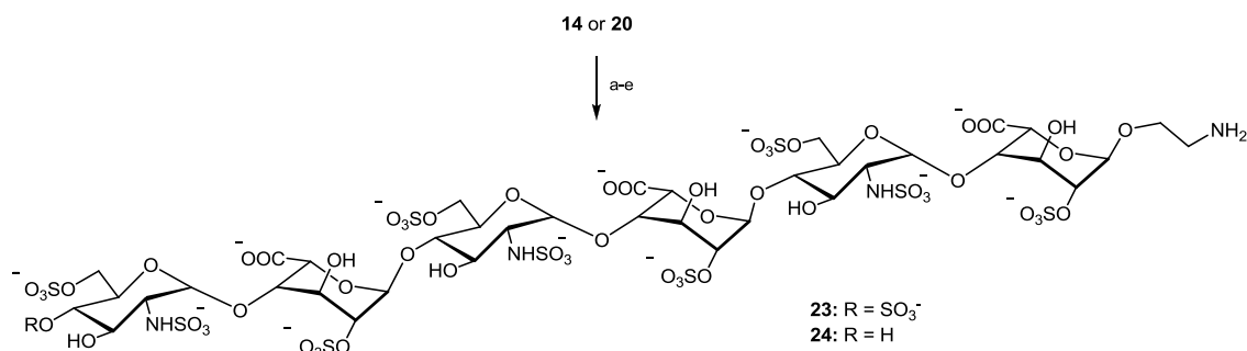
Scheme 7. Synthesis of hexasaccharides 23 and 24 . Reaction conditions: a) LiOH, H 2 O 2 , THF; NaOH, MeOH; b) SO 3 ·Me 3 N, DMF, 100°C, MW; c) Me 3 P, THF, NaOH; d) SO 3 ·Me 3 N, DMF, Et 3 N, 60°C, MW; e) H 2 , Pd(OH) 2 , H 2 O/MeOH, 23 , 30%; 24 , 13%, five steps.
