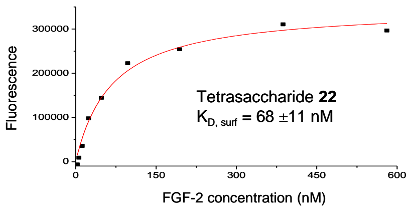
Figure 2. Binding curves for oligosaccharides 22 , 23 and 24 . Average fluorescence intensities of five replicates were plotted against FGF-2 concentrations. The K_{D, surf} values were obtained by fitting the curves to a Langmuir isotherm for a one-site model of interaction.
