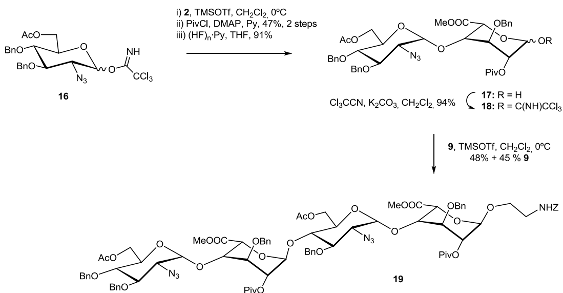
Scheme 5. Synthesis of tetrasaccharide derivative 19 .
