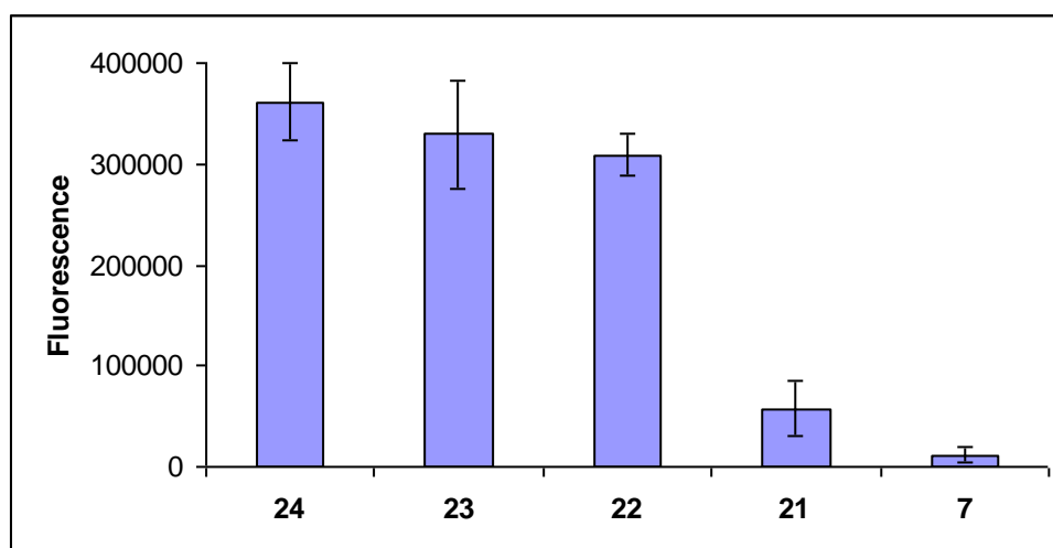
Figure 1. Binding of synthetic heparin-like oligosaccharides to FGF-2. Sugar-coated wells were incubated with 291 nM protein. For each oligosaccharide, fluorescence signals are the average of five replicate wells and the error bars show the standard deviations for these measurements.
