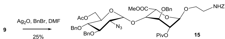
Scheme 4. Benzylation of disaccharide 9 .
