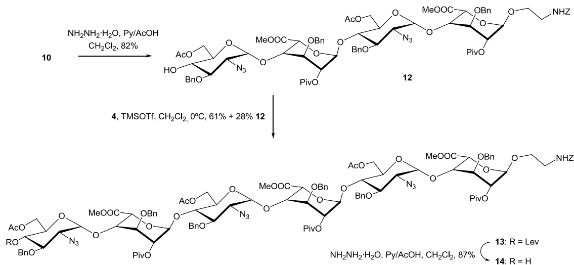
Scheme 3. Synthesis of hexasaccharide intermediate 14 .
