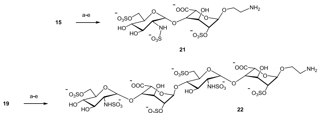
Scheme 6. Synthesis of disaccharide 21 and tetrasaccharide 22 . Reaction conditions: a) LiOH, H 2 O 2 , THF; NaOH, MeOH; b) SO 3 ·Me 3 N, DMF, 100°C, MW; c) Me 3 P, THF, NaOH; d) SO 3 ·Py, Py, Et 3 N; e) H 2 , Pd(OH) 2 , H 2 O/MeOH, 21 , 45%; 22 , 36%, five steps.
