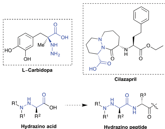
Fig. 1 Hydrazino acids in medicinal chemistry.
