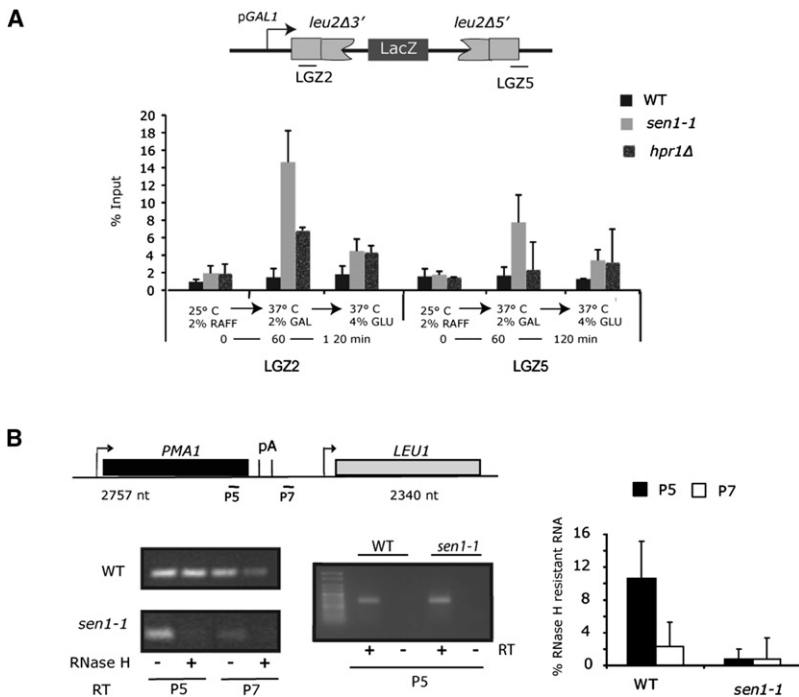
Figure 4. R Loops Form in sen1-1 Cells
