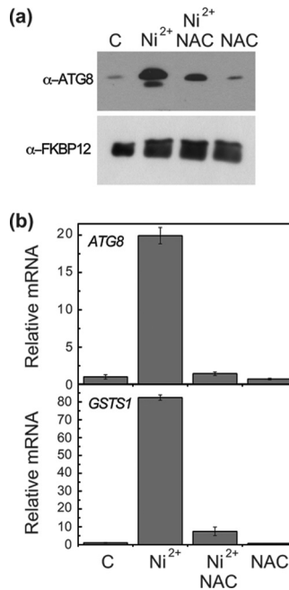
FIG 6 Effect of the antioxidant NAC on Ni 2+ -induced autophagy. The protein abundance and lipidation of ATG8 (a) and the accumulation of ATG8 and GST 1 gene transcripts (b) in Chlamydomonas cells treated with 100 \mu M Ni 2+ for 8 h in the presence or absence of 10 mM NAC were determined. (a) Immunoblot analysis with an anti-FKBP12 antibody was used as loading control. (b) mRNA levels were determined by qPCR and normalized to those for control cells (for which the level of mRNA expression was given a value of 1). The data are represented as the mean \pm standard deviation from three independent experiments.
