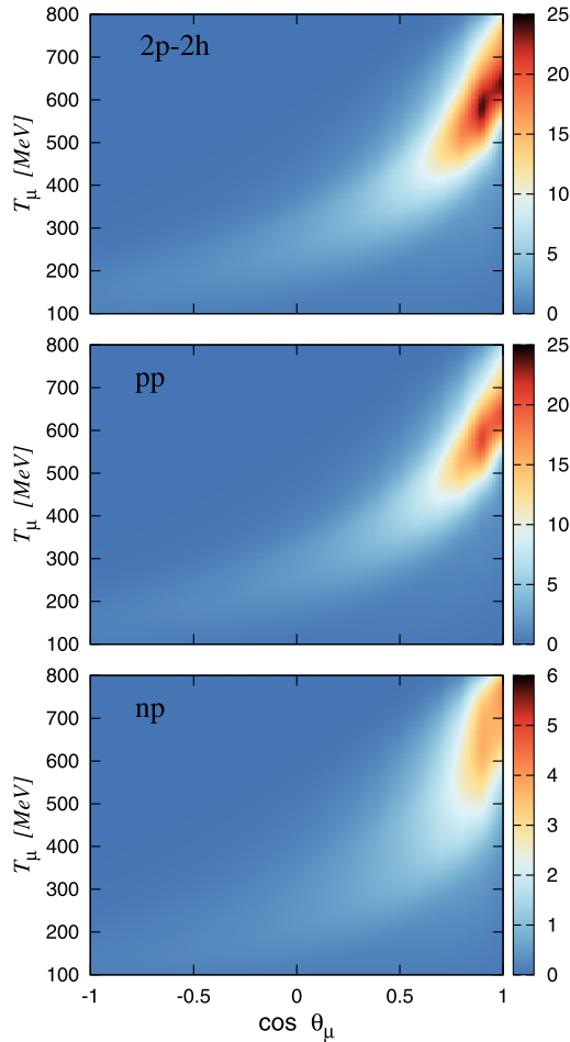
Fig. 8. (Color online.) Double differential 2p-2h neutrino cross section per neutron of ^{12}\text{C} , d^2\sigma/d\cos\theta_\mu dT_\mu/N , in units of 10^{-39} \text{ cm}^2/\text{GeV} , as a function of \cos\theta_\mu, T_\mu for fixed neutrino energy E_\nu = 1 \text{ GeV} . The separate pp and np channels are shown in the middle and bottom panels, respectively.
