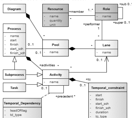
Fig. 4. BPMN metamodel extensions.
