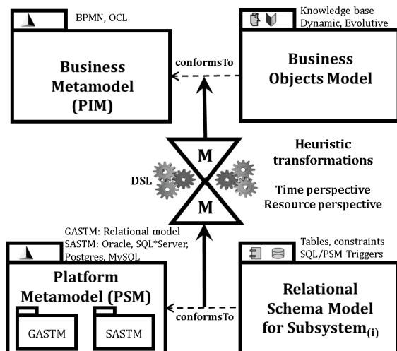
Fig. 5. Reverse engineering from PSM to PIM.
