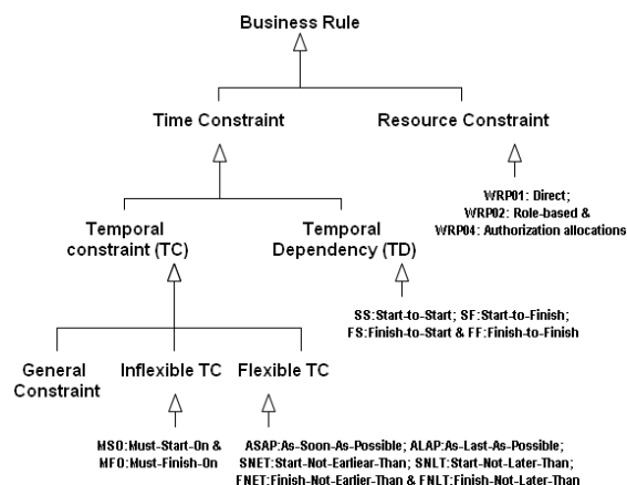
Fig 2. Business rules taxonomy.
