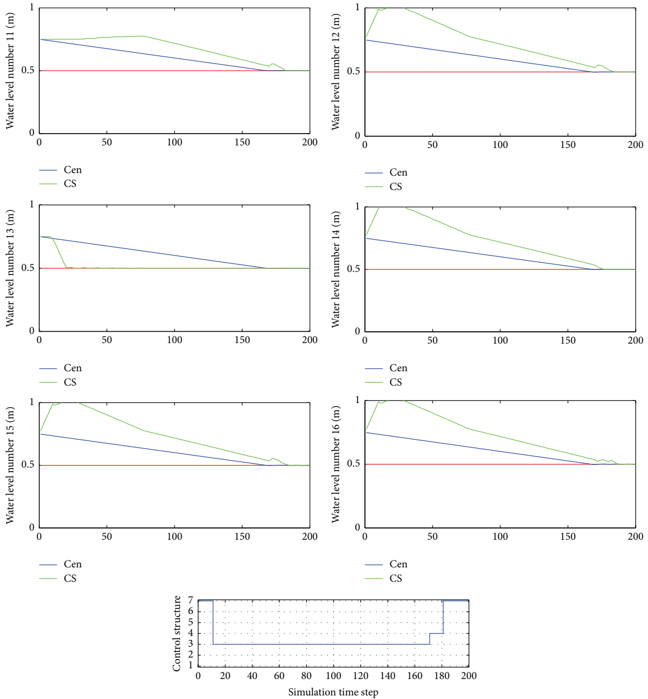
FIGURE 7: Evolution of the water levels of all the tanks and the control structure when the initial state is 0.75 m for all the tanks. The x -axis corresponds to the simulation step. The reference is 0.5 m. Cen is the Centralized MPC solution; CS is the proposed NC-MPC method. Red represents reference.
