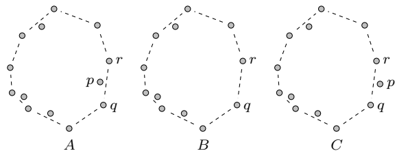
Fig. 2. The point sets A, B and C . Here v = 9 and i = 4 .
