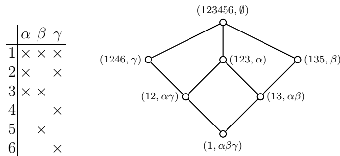
Fig. 2. The incidence table of \mathcal{C} (left) and its concept lattice (right)
