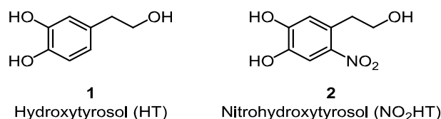
Figure 1. Chemical structures of parent compounds (1) and (2).
