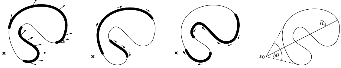
Figure 1. From left to right: rotated exit boundary regions in a domain corresponding to \theta = 0 , \theta \rightarrow \pi/2 and \theta \rightarrow -\pi/2 with respect to some exterior point x_0 . The last figure shows the main geometrical parameters of the problem.
