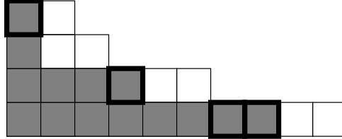
FIGURE 1. The horizontal strip H (boxes with thick edges) for \kappa = (10, 6, 3, 2) (white and grey boxes) and \delta = (8, 4, 1, 1) (grey boxes).
