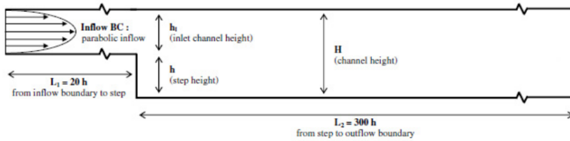
Figure 2: Geometric characteristics of backward-facing step problem
