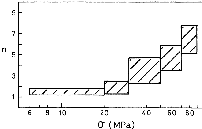
Fig. 3. — Stress exponents n versus applied stresses \sigma at temperatures between 1 100 °C and 1 500 °C in P_{O_2} of 0.21 atm and 10^{-5} atm.
