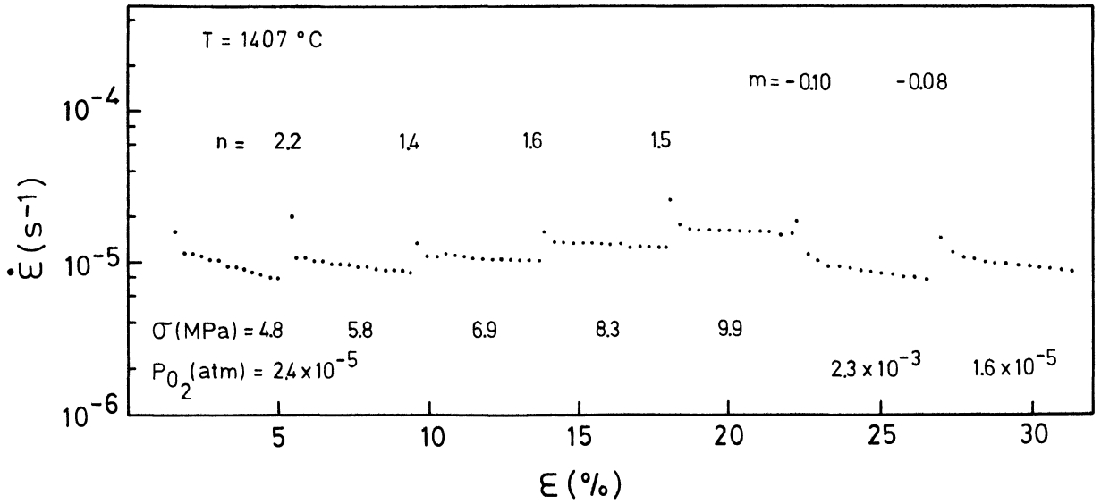
Fig. 2. — Compression creep curve of a NiO polycrystal with 6% porosity and 8 μm grain size. Stress and P_{O_2} changes have been performed.
