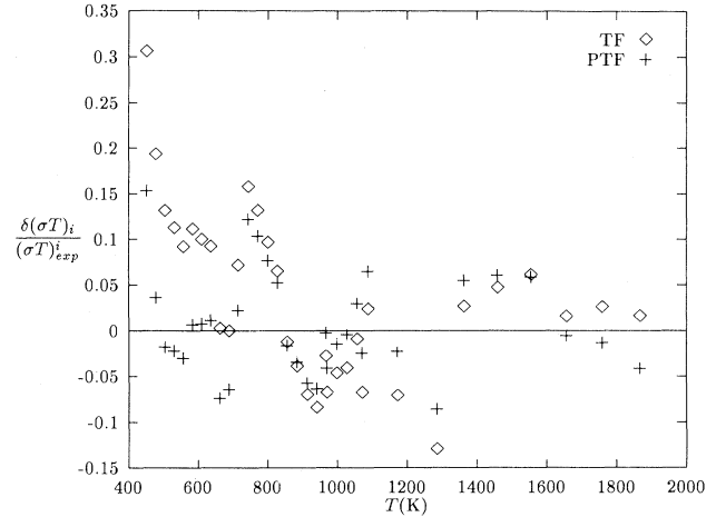
FIG. 4. Relative fitting errors found by applying the TF ( \diamond ) and PTF ( + ) procedures to the \sigma T data measured in 12 mol% Y-FSZ single crystals.
