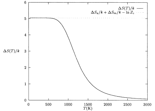
FIG. 3. Temperature behavior of the \Delta S(T) function. It has a similar shape to \Delta H(T) , although with a sharper drop. The extrinsic associated range is marked as (\frac{\Delta S_a}{k} + \frac{\Delta S_m}{k} - \ln Z_c) .
