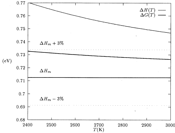
FIG. 1. Magnification of the asymptotic high-temperature behavior of \Delta H(T) and \Delta G(T) . One sees that the differences between \Delta G(T) and \Delta H_m are less than 3% from 2400 K to the melting point.
