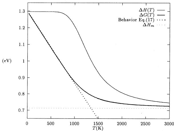
FIG. 2. Temperature behavior of the \Delta H(T) and \Delta G(T) functions. On the same plot are \Delta G(T) in the extrinsic associated range [Eq. (17)] and the asymptotic high-temperature value, \Delta H_m .
