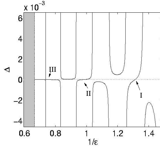
Figure 10: Continuation of weakly non-local solitons for various values of 1/\varepsilon showing three zeros in \Delta for c = 0.7 , \Lambda = 0.5 , L = 60 . Zeros of \Delta at \varepsilon \approx 0.76, 1.02, 1.36 . The shaded region represents the spectral band where any embedded solitons would be of co-dimension 2.
