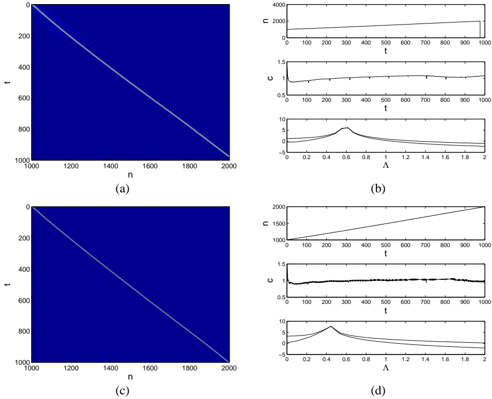
Figure 18: Direct integration of a perturbed solution from Branch I in Figure 13 with \varepsilon = 1 and c = 1.00926 , \Lambda = 0.5 , N = 2000 . (a) Motion of the solution with \alpha = 0.8 through the lattice for 1000 time steps, (b) the top panel shows the position of the soliton at time t , the middle panel shows the velocity based upon numerical differentiation, and the lower panel shows the log of the power spectrum indicating a shift in frequency from the unperturbed value \Lambda = 0.5 . (c) and (d) show the same as (a) and (b) but with \alpha = 1.2
