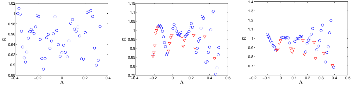
Figure 26: Dependence of the restitution coefficient for collisions of a travelling wave with c = 1.3006 and \Lambda = 0.0143 in branch I (left), c = 1.0338 and \Lambda = 0.1129 in branch II (center) and c = 0.8881 and \Lambda = 0.0845 in branch III (right). These collisions take place with waves of the same branch whose \Lambda is indicated in the X-axes of the graphs. Circles correspond to reflection / refraction and triangles to breather creation.
