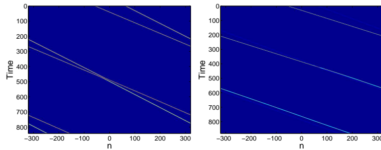
Figure 29: Collision of two traveling waves with different velocities moving in the same direction. They have (Left) c = 1.4201 and \Lambda = -0.3509 , belonging to branch II and c = 1.1804 and \Lambda = -0.1817 , belonging to branch III. The coherent structures repel each other. (Right) c = 1.6433 and \Lambda = -0.5597 , belonging to branch I and c = 1.1804 and \Lambda = -0.1817 , belonging to branch III. The waves are refracted.
