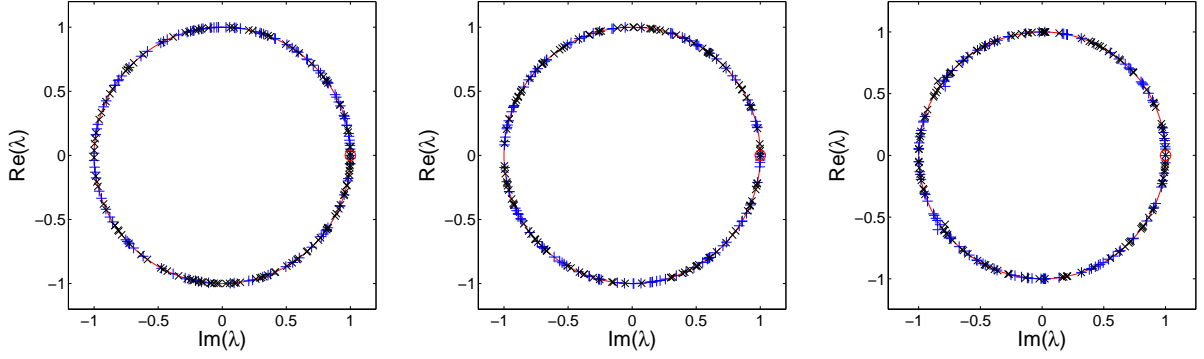
Figure 22: Floquet eigenvalues in the unit circle. Solutions corresponds, from left to right, to the 1st, 2nd and 3rd branches. In all cases, q = 8, p = 1 . The Krein signature (see e.g., [19], [3]) is indicated by the following signs: Positive (+), negative (×) and zero ○
