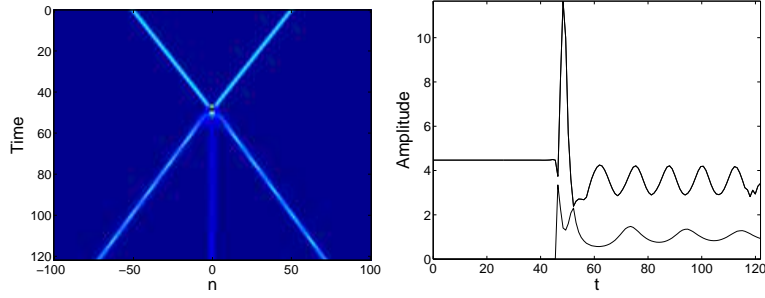
Figure 25: Collision of two waves with initial velocity c = 1.0338 and \Lambda = 0.1129 . They are refracted / reflected after the collision with an extra breather created. The panels are similar to those of Fig. 24, but the right panel also shows the amplitude of the wave created at n = 0 .
