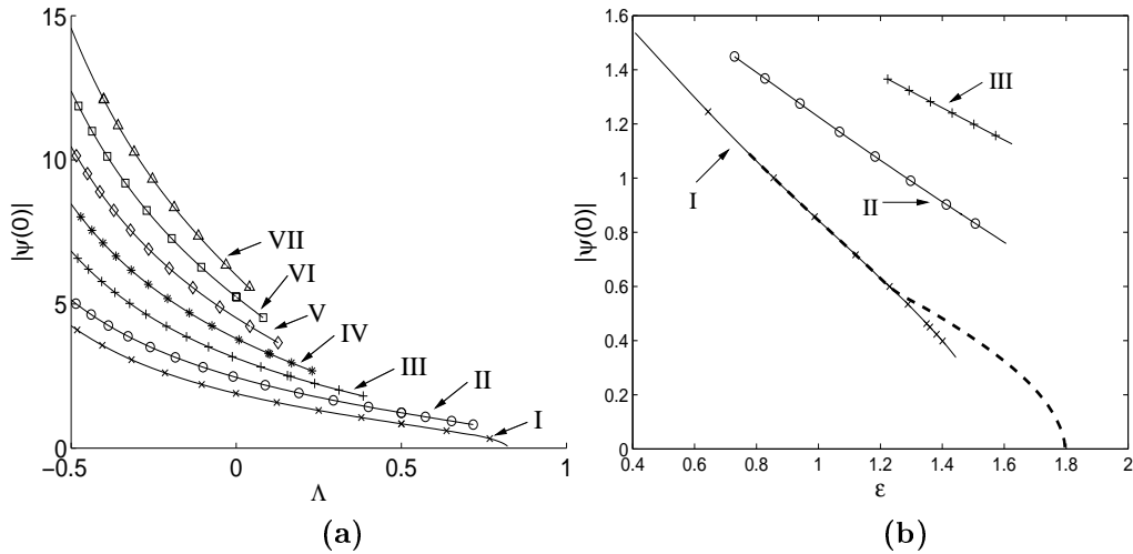
Figure 16: Amplitude of solutions, |\psi(z = 0)| along the continuation branches shown in (a) Figure 15 as \Lambda varies and (b) from Figure 13 as \varepsilon varies. Thick dashed line in panel (b) is from a solution on Branch I for which \psi_{core} \neq 0 in the tail hence L is too small, however this gives a good indication that the soliton amplitude goes to zero as it intersects the upper phonon band.
