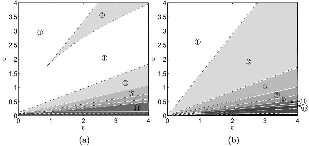
Figure 3: Intersections of (7) and (8) for \Lambda = 0.5 and varying c and \varepsilon . The shaded areas show regions where there is more than one branch of linear waves according to (7) & (8). Values indicate the number of roots of (7) in each region. Subplots show left and right hand sides of (7) for (\varepsilon, c) = (1, 3) , one root (i), (3, 3.5) , three roots (ii) and (3.5, 0.6) , seven roots (iii). (iv) displays the overlapping of the bands for small \varepsilon, c , only the first six bands have been shown.
