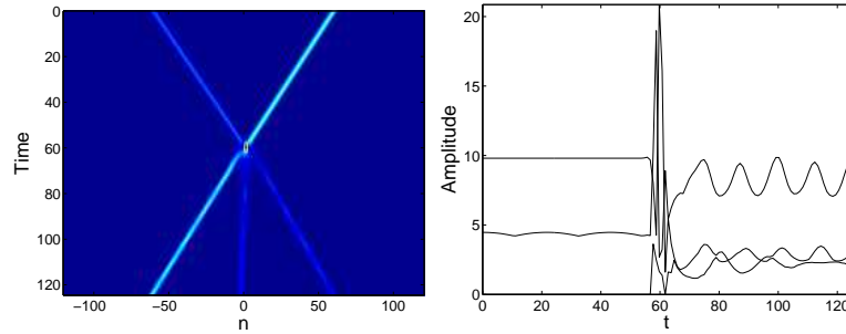
Figure 28: Collision of two waves with different velocities. One belongs to branch II with initial velocity c = 1.0338 and \Lambda = 0.1129 . The other one belongs to branch III, having initial velocity c = 0.9876 and \Lambda = -0.0025 . The panels are similar to the previous figure.
