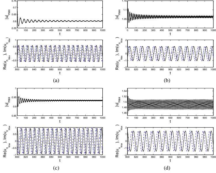
Figure 20: Profiles of perturbed embedded solitons, (a) Branch I soliton with \alpha = 0.8 , (b) Branch I soliton with \alpha = 1.2 , (c) Branch II soliton with \alpha = 0.8 , (d) Branch II soliton with \alpha = 1.2 . Top panels show |u| for soliton and bottom panels. Re(u) - solid line, Im(u) - dashed line.
