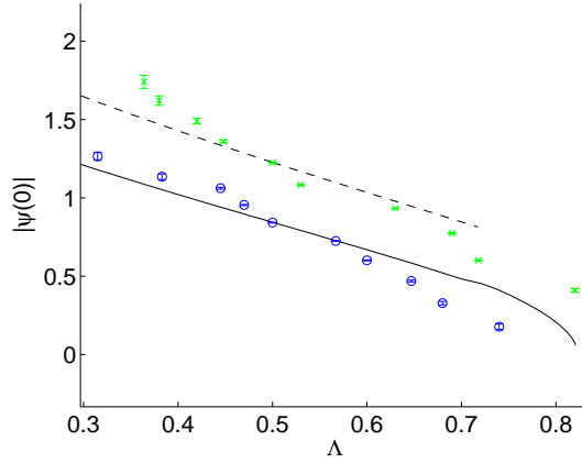
Figure 21: Change in frequency, \Lambda , of a soliton due to perturbation of the initial profile with \Lambda = 0.5 , \alpha \in (0.5, 1.4) . Branch I, solid line indicates unperturbed solution amplitudes, with perturbed solutions shown by circles. Branch II, dashed line indicates unperturbed solution amplitudes, perturbed solutions indicated by crosses. Error bars indicate the variation in amplitude.
