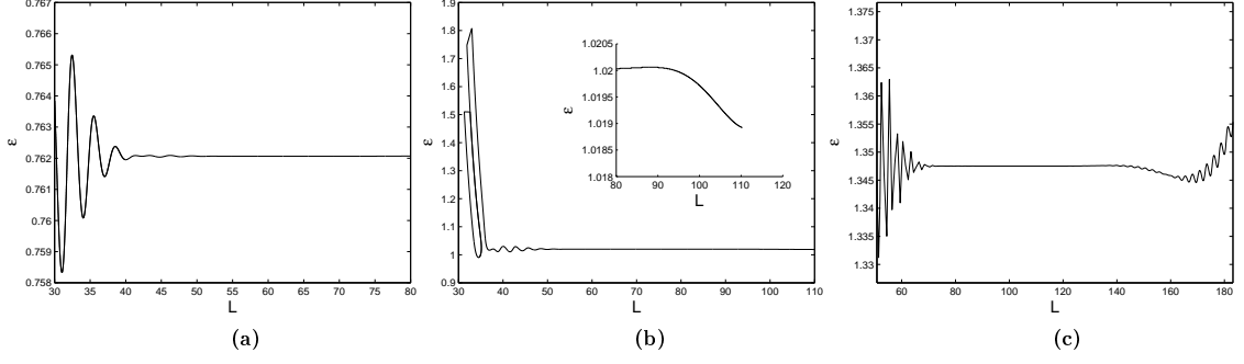
Figure 8: Continuation of three zeros of \Delta in L and \varepsilon with c = 0.7 , \Lambda = 0.5 with N = 200 (a) & (b) and N = 300 (c). The inset shows the variation in \varepsilon for large \Delta due to the value of N being taken too small. (a) belongs to Branch I, (b) to Branch II, and (c) to Branch III, in the notation used below.
