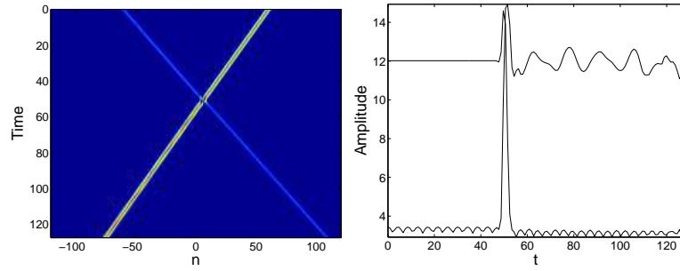
Figure 27: Collision of two travelling waves of different velocities. One belongs to branch I with initial velocity c = 1.3006 and \Lambda = 0.0143 . The other one belongs to branch III, having initial velocity c = 1.0676 and \Lambda = -0.0751 . They are refracted / reflected after the collision. (Left) The space-time contour plot of the density is shown. (Right) The time dependence of the amplitude of the traveling waves is presented.
