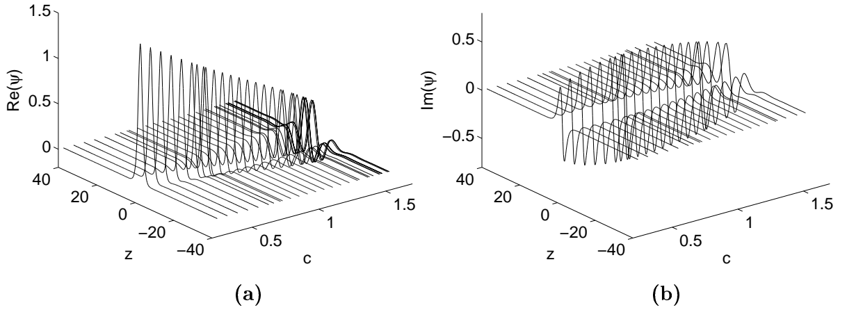
Figure 14: Continuation of the first branch of solutions with varying \varepsilon , c and \Lambda = 0.5 (a) Re(\psi(z)) , (b) Im(\psi(z)) . The lower portion of the branch is computed with L = 60 , if the solution is continued inside the multi-phonon band it becomes delocalized. As c is increased larger values of L = 80 and 280 are used to capture the solution as the soliton core expands. Near the upper phonon band the soliton branch terminates. Solutions have been truncated in z for ease of viewing.
