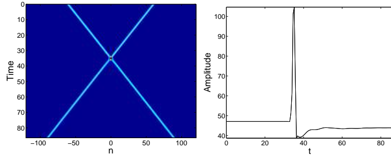
Figure 24: Collision of two solitary waves belonging to branch I with initial velocity c = 1.7351 and \Lambda = -0.7121 . They are refracted / reflected after the collision. (Left) Space-time contour plot of the solution density. (Right) Time dependence of the amplitude of the moving wave.
