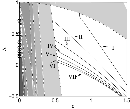
Figure 15: Continuation of the 3 solitary wave branches with varying \Lambda and c for fixed \varepsilon = 1 . Extra branches, labelled IV - VII are also found for smaller values of \Lambda . Branches appear to converge in the large wavespeed limit.
