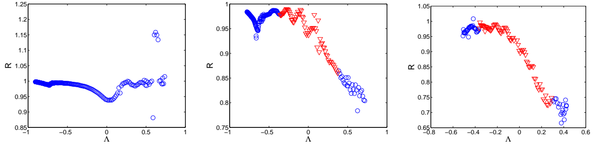
Figure 23: Dependence of the restitution coefficient for symmetric collisions with respect to the frequency \Lambda for branches I, II and III (from left to right). Circles correspond to reflection / refraction and triangles to breather creation.
