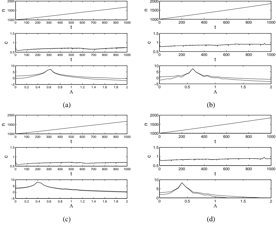
Figure 19: Variation in position, wavespeed, c and frequency \Lambda for perturbed solutions on branch II with (a) \alpha = 0.8 and (b) \alpha = 1.2 . Branch III with (c) \alpha = 0.8 and (d) \alpha = 1.2 . Panels are the same as for Figure 18 (b) and (d).
