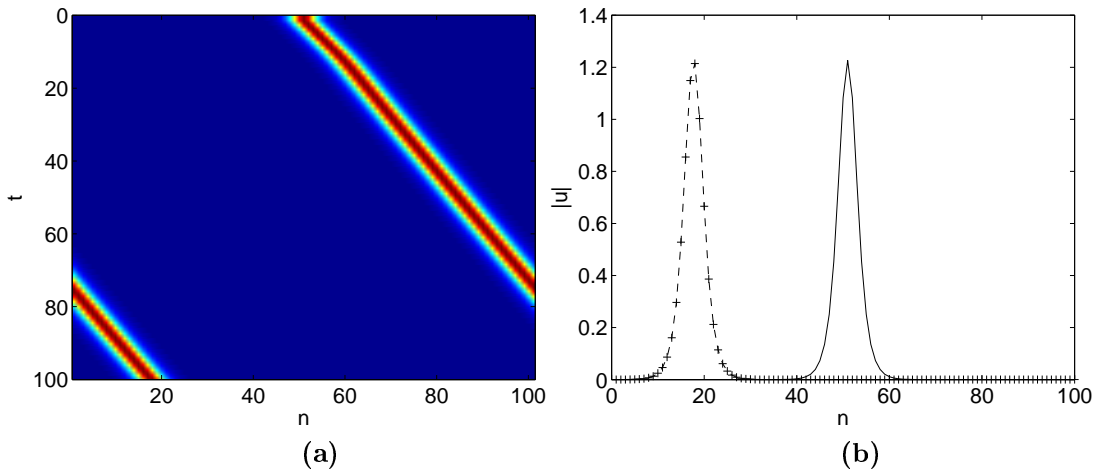
Figure 17: Numerical Integration of the solution of Branch II in Figure 13 with \varepsilon = 1 , c = 0.67725 with \Lambda = 0.5 , N = 100 . (a) Motion of the solution through the lattice for 100 time steps (shown is a space-time contour plot of the modulus of the solution), (b) Initial and final profiles of the wave after 100 time steps; the final lattice node points are indicated with a +.
