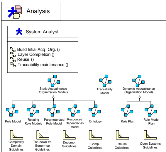
Fig. 1 Acquaintance analysis discipline
