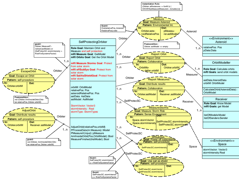
Fig. 9 Composed Role Model
