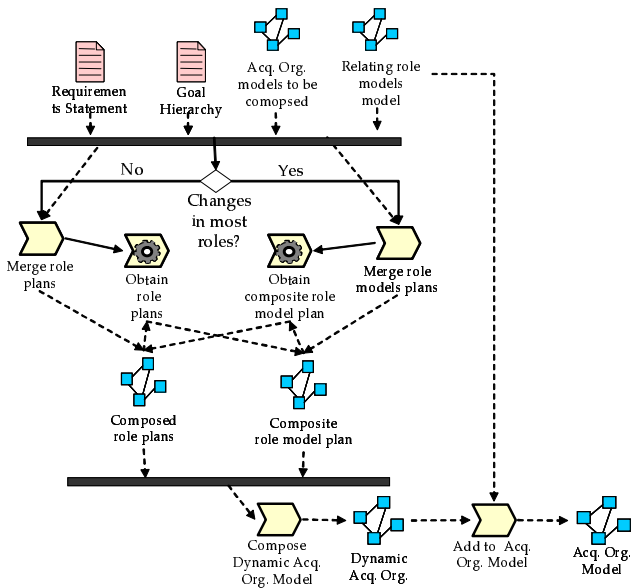
Fig. 8 Software Process of Plan Composition
