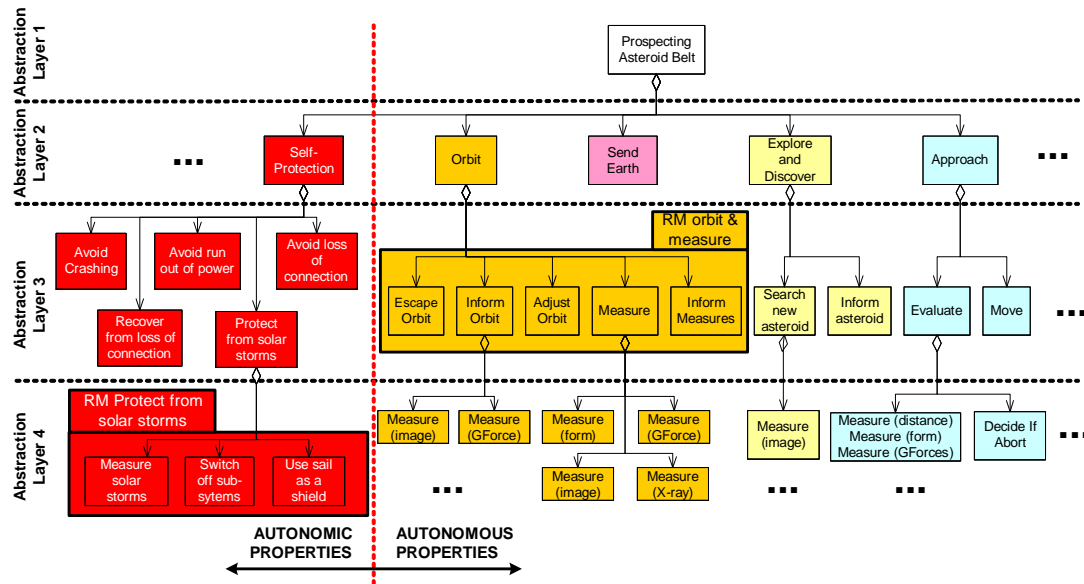
Fig. 3 Traceability model of ANTS
