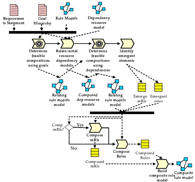
Fig. 7 Software Process of Role Composition
