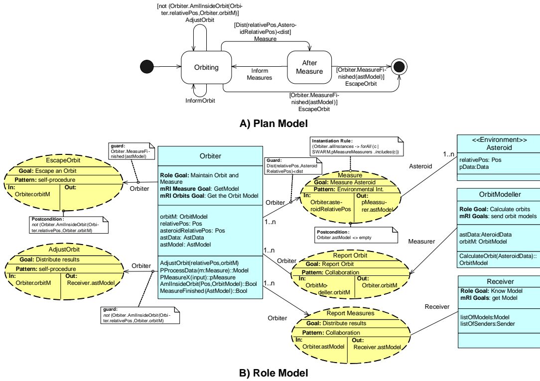
Fig. 4 Orbiting and measuring an asteroid autonomous property
