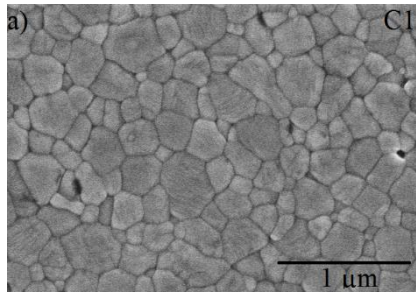
Figure 3. SEM micrographs of polished cross sections after annealing in air to show 3YTZP grain boundaries. a), b), c), d) and e) correspond to C1, C2, C3, C4 and C5 composites respectively.
