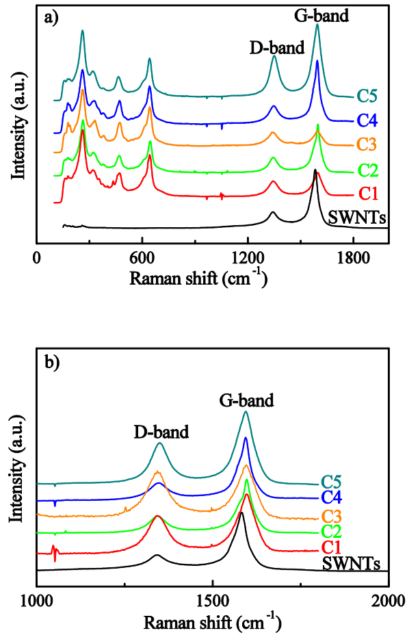
Figure 4. Raman spectra from the 3YTZP / 1 vol% SWNT composites sintered in this study. (a) Spectra normalized to the 3YTZP peaks and (b) area of interest normalized to the G-band for easier comparison.
