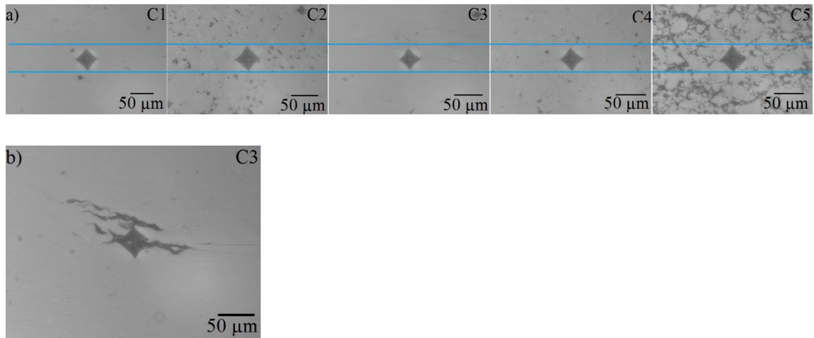
Figure 5. a) Optical micrographs showing Vickers indentations (1.96 N) on cross sections of the studied composites. b) Non symmetric Vickers imprint on a large SWNT agglomerate in composite C3.
