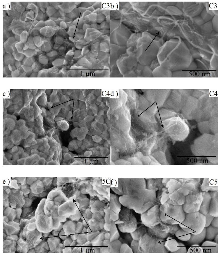
Figure 2. Fracture surfaces of composites C3, C4, and C5, showing ceramic 3YTZP grains and SWNTs (arrowed) at different magnifications.
