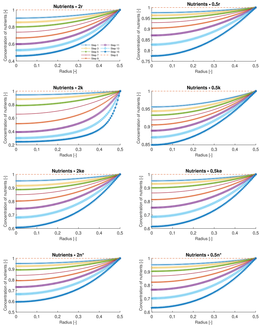
Fig. 6. Parametric analysis of the distribution of the concentration of nutrients along the dimensionless radius of the spheroid, at time steps 0, 1, 3, 5, 7, 9, 11, 13 and 15, for cases 2r, 0.5r, 2k, 0.5k, 2ke, 0.5ke, 2n* and 0.5n*.
