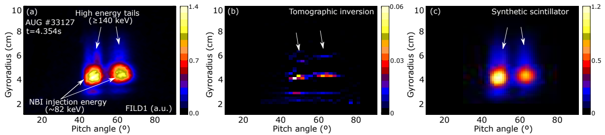
Figure 1: (a) Velocity-space measurement of fast-ion losses during an ELM. (b) Tomographic reconstruction of the undistorted velocity-space distribution reaching the detector pinhole. (c) Synthetic FILD signal obtained after the tomographic inversion.
