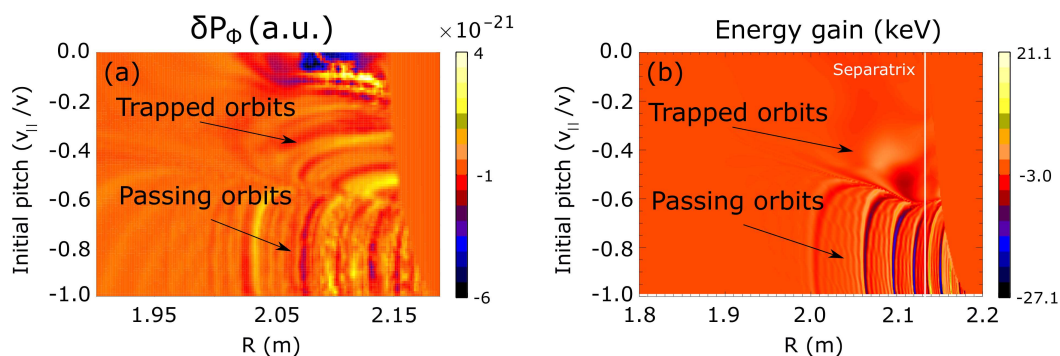
Figure 2: (a) Variation of P_{phi} in the presence of the 3D magnetic perturbation fields calculated with JOEREK. (b) Energy gain in the presence of the test model for the parallel electric field.
