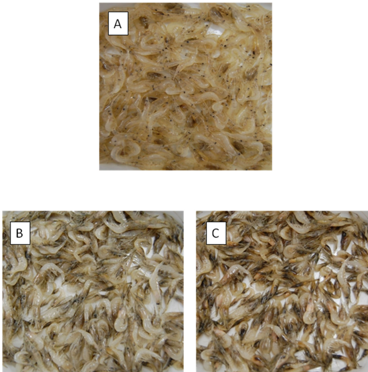
Figure 2. Atlantic ditch shrimp treated for 10 min with 10 \mu\text{M} of diselenide of bis-HT. (A) shrimp before the treatment, (B) treated shrimp after 5 days of refrigerated storage at 4–6 ^{\circ}\text{C} , (C) untreated shrimp after 5 days of refrigerated storage at 4–6 ^{\circ}\text{C} .
