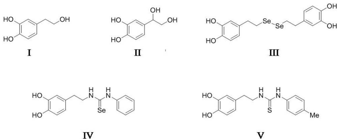
Figure 1. Chemical structures of hydroxytyrosol (HT) (I), 3,4-dihydroxyphenylglycol (DHPG) (II), dihydroxytyrosyl diselenide (diselenide of bis-HT) (III), N-hydroxytyrosyl selenourea (selenourea) (IV), and N-hydroxytyrosyl thiourea (thiourea) (V).
