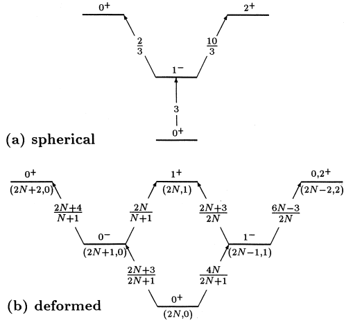
Fig. 1. E1 excitation patterns up to (\text{GDR})^2 in (a) the spherical weak-coupling limit and (b) the deformed strong-coupling limit. (a) The levels are labelled by J^\pi on top. The numbers between levels are the strengths B(E1; (n,0)J \rightarrow (n+1,0)J') in units of \zeta^2 . (b) The levels are labelled by (\lambda, \mu) underneath and by K^\pi on top. The expressions between levels are the summed strengths \sum_{K'L'} B(E1; (\lambda, \mu)KL \rightarrow (\lambda', \mu')K'L') in units of \zeta^2 .
