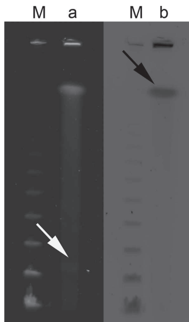
FIG 1 Southern blot assay. Lane a, PFGE analysis of the AB 308 strain by digestion with S1 nuclease. Lane b, hybridization with a bla OXA-23 probe. The black arrow indicates the chromosomal location with positive hybridization with the bla OXA-23 probe. The white arrow indicates a plasmid band with no hybridization with the probe. Lanes M, lambda ladder PFGE marker (New England BioLabs).
