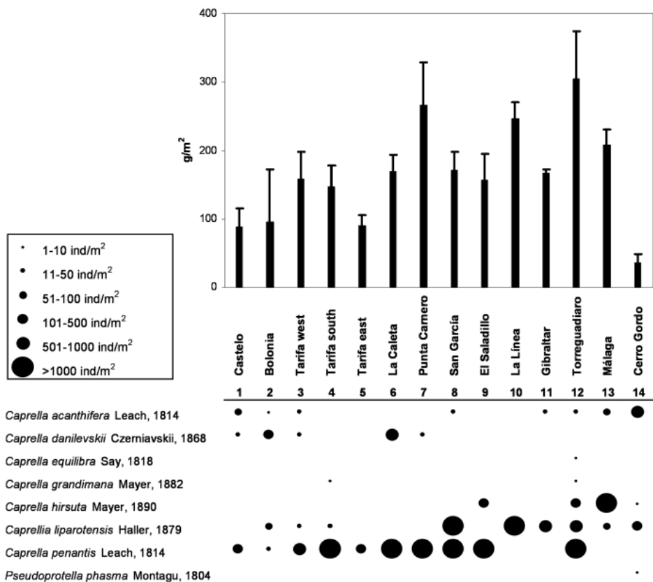
Fig. 4.—Caprellid densities measured in the fourteen stations considered. The histogram represents the A. armata biomass ( \text{g}/\text{m}^2 ) in each station. Values of biomass are mean \pm standard deviation.
