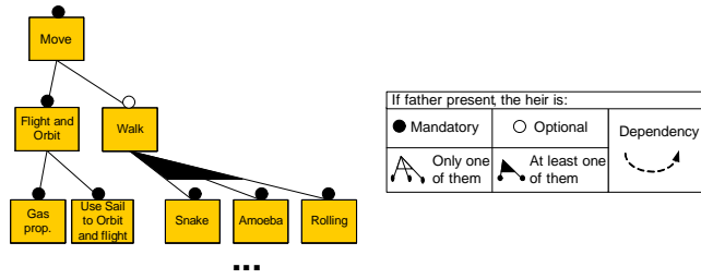
Fig. 1. Sub-set of the feature model of our case study
