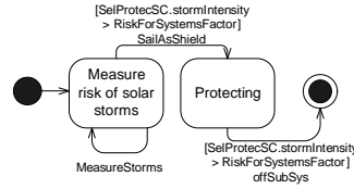
A) Plan Model
