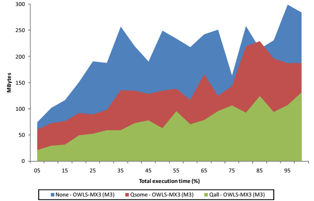
Figure 4: Memory consumption statistics when filtering OWLS-MX3 (M3).
