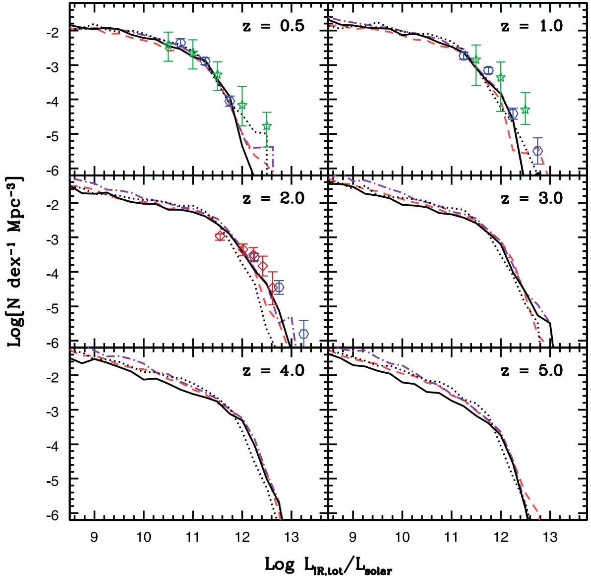
Figure 12. LFs for the total IR emission. Line types are the same as in Fig. 9; however as the total IR predictions are insensitive to the templates used, the model with the DGS99 templates is not shown. Blue hexagons are the data from Rodighiero et al. (2010), green stars are from Le Floc'h et al. (2005) and red diamonds are from Caputi et al. (2007).
