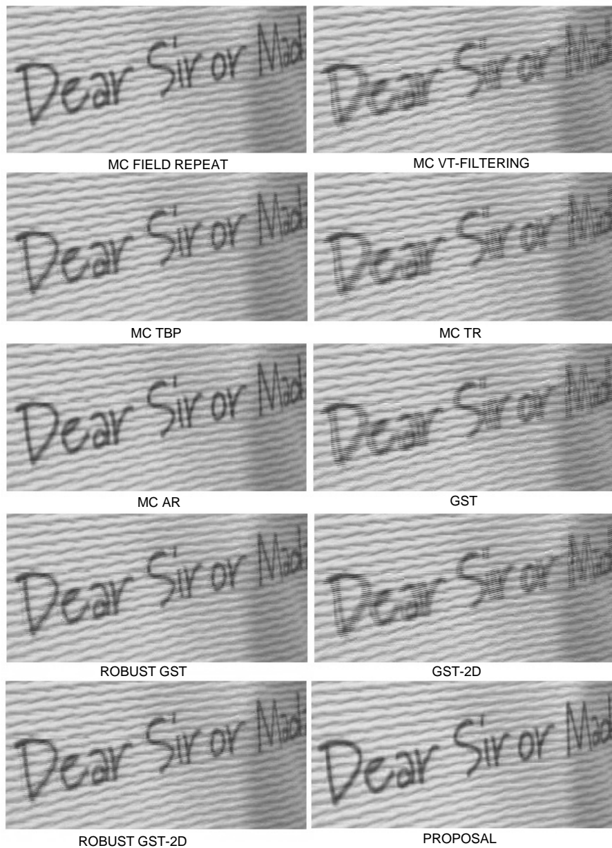
Fig. 13. Deinterlaced images obtained with MC de-interlacing algorithms and our proposal in the Paper 3D hybrid sequence.
