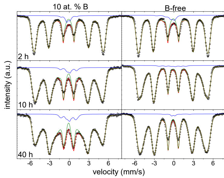
Figure 4. Mössbauer spectra. Symbols correspond to experimental data and lines to the total fitting as well as to the two HFD used (Color online).
