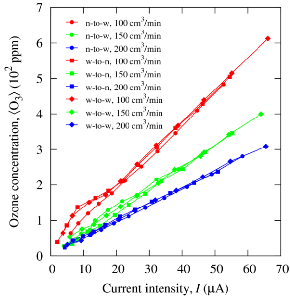
Fig. 5. Ozone concentration as a function of the current intensity (negative corona) for different gas flow rates and flow directions. n-to-w : needle (entry) to lateral port (exit), w-to-n : lateral port (entry) to needle (exit), w-to-w : lateral port (entry) to opposite lateral port (exit).
