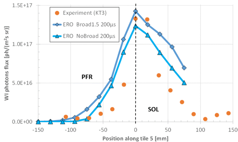
Fig. 8. Simulated profiles of WI emission along tile 5 during ELM in comparison with the measured one. An effective ELM duration of 200 \mu\text{s} has been applied in the simulations. Simulated profiles are shown with (Broad1.5) and without (NoBroad) broadened decay lengths for the plasma parameters.
