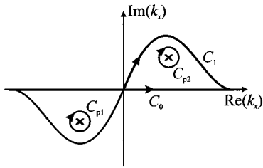
Fig. 2. Paths of integration in the complex k_x -plane. For simplicity, only a pair of surface-wave poles are shown (x).
