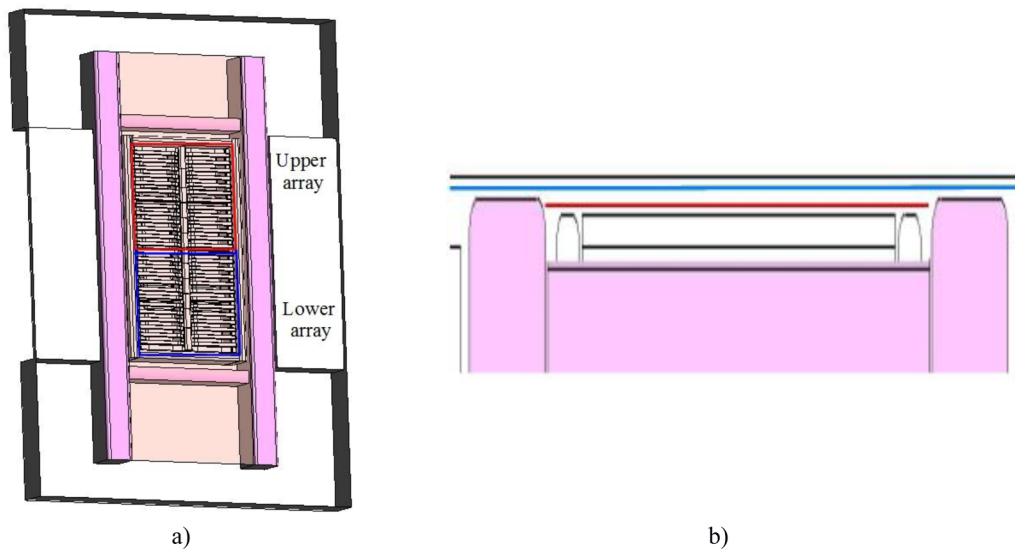
Fig. 1. a) Flat model of the ILA, b) side view (zoomed and elongated) with limiters and antenna frame, vacuum-plasma boundary is in black, first surface or E_{\parallel} calculations above the limiters is in blue, surface for E_{\parallel} calculations between the limiters is in red (corresponding to x = 0 on Fig. 5). (For interpretation of the references to color in this figure legend, the reader is referred to the web version of this article.)
