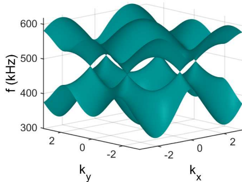
FIG. 1: Typical band structure of the infinite honeycomb lattice in the first Brillouin zone. There are six Dirac points corresponding to (k_x, k_y) = (0, \pm 4\pi/(3\sqrt{3})), (2\pi/3, \pm 2\pi/(3\sqrt{3})), (-2\pi/3, \pm 2\pi/(3\sqrt{3})) and a frequency f_d = 489.11 kHz, cf. Eq. (5).
