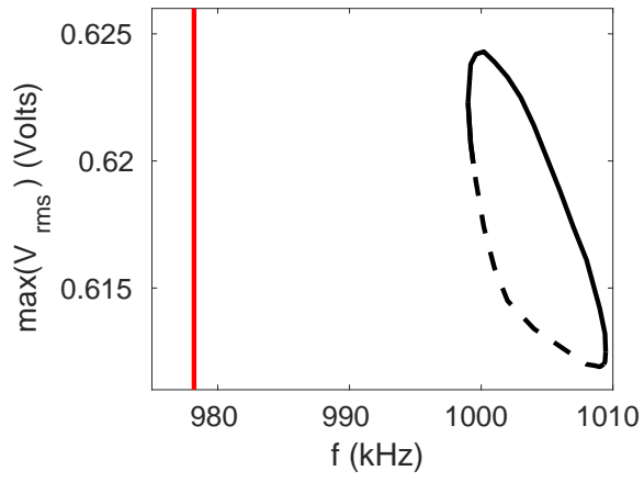
FIG. 9: V_{\text{rms}} on peak node of the numerically calculated subharmonic EBs (solutions in red and blue at Fig. 8), as a function of the frequency. Stable solutions are depicted as continuous lines and unstable solutions as dotted lines. The red line marks twice Dirac frequency ( 2f_d ).
