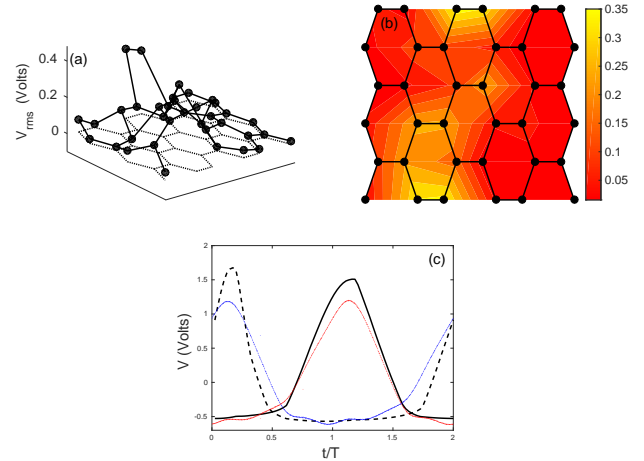
FIG. 7: (a) Experimental subharmonic armchair-EB profile in a 6 \times 6 lattice with free boundaries and (b) its corresponding density plot. The square-wave driving amplitude was set to 9 V and the frequency to 886 kHz. (c) Time dependence of the voltage at the two largest amplitude nodes on the top of the lattice: numerical simulations are shown by black continuous and dashed lines, whereas experimental data are shown in blue and red lines.
