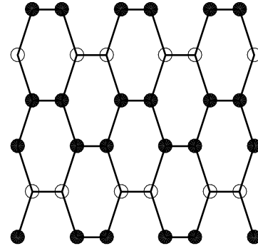
FIG. 2: Finite size ( 6 \times 6 ) lattice with free boundaries; shown is the Dirac mode, i.e. the linear mode corresponding to f = f_d = 489.11 kHz. Black and white circles correspond, respectively, to a normalized amplitude in t = 0 of 1/2 and -1 .
