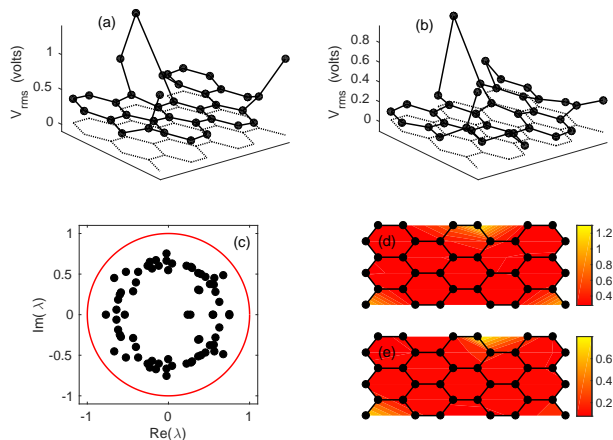
FIG. 4: Same as figure 3 but for an edge breather (EB) in a free-boundary lattice.
