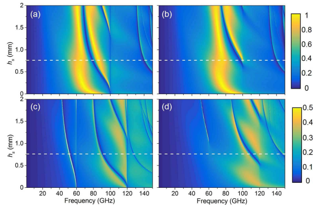
Fig. 6. ECA results of the transmission coefficient for FSS and ET designs versus frequency and h_s . (a) FSS—vertical polarization ( \varphi = 90^\circ ). (b) FSS—horizontal polarization ( \varphi = 0^\circ ). (c) ET—vertical polarization ( \varphi = 90^\circ ). (d) ET—horizontal polarization ( \varphi = 0^\circ ). Horizontal white dashed lines denote the particular cases shown in Fig. 5.
