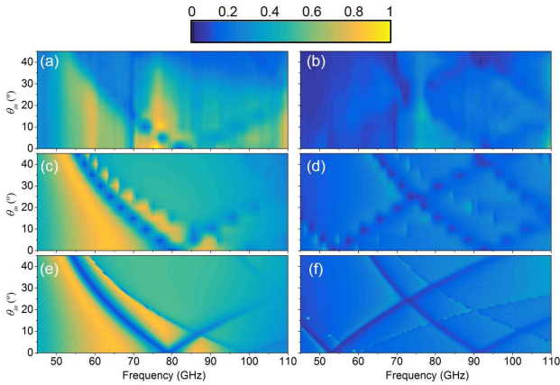
Fig. 12. Transmission coefficient versus frequency and \theta_{in} for TM polarized impinging wave and \varphi = 90^\circ incidence plane for FSS and ET prototypes. (a) Experiment—FSS. (b) Experiment—ET. (c) CST—FSS. (d) CST—ET. (e) Equivalent circuit—FSS. (f) Equivalent circuit—ET.
