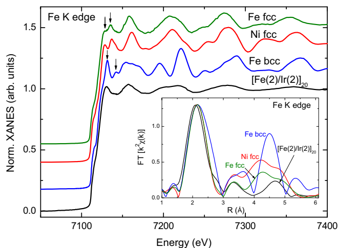
FIG. 2. Fe K-edge XAS spectra recorded on [Fe(2)/Ir(2)] 20 and bulk Fe, bulk Ni, and fcc-Fe nanoparticle [35] references. The inset shows the modulus of the Fourier transforms of the k^2 -weighted EXAFS signals in the range from 3 Å -1 to 10 Å -1 . For the sake of a better comparison the FT of the references has been multiplied by a factor of 0.3.
