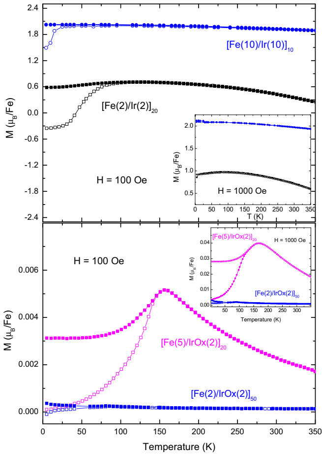
FIG. 9. FC and ZFC magnetothermal curves.
