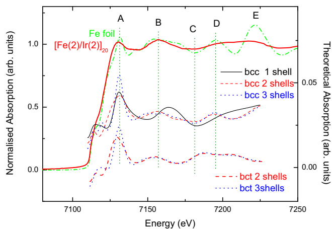
FIG. 3. The Fe K-edge XANES spectra recorded on the [Fe(2)/Ir(2)] 20 sample are compared to the theoretical spectra obtained for Fe bcc clusters.
