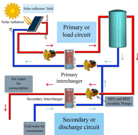
Fig. 3. General scheme
