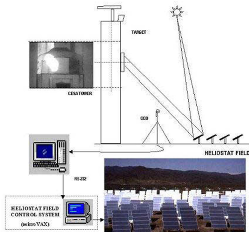
Fig. 2. Heliostat calibration
