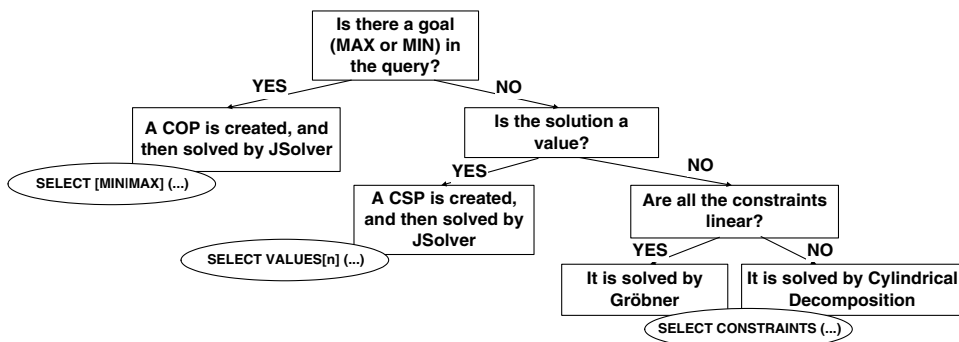
Fig. 9. Decision tree to choose what part of the architecture to use.
