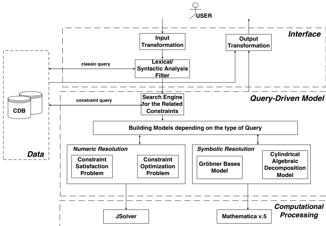
Fig. 8. Labelled object-relational CDB architecture for projection.
