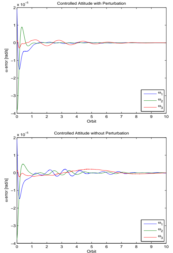
Figure 4. Angular velocity error
