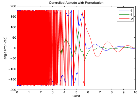
Figure 8. Angle error
