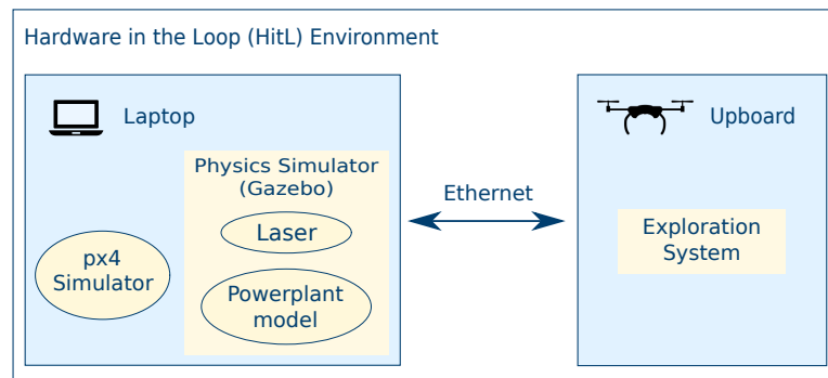
Figure 8. The diagram of the Hardware-in-the-Loop (HitL) environment details how the load balancing between the Upboard and the support laptop reflect the resources available in a real flight.
