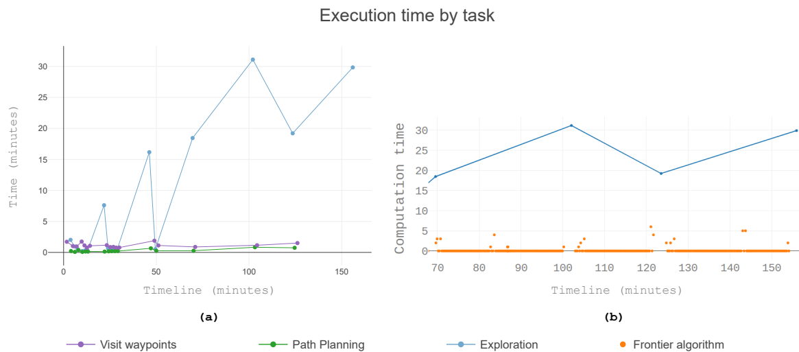
Figure 10. Time used in exploration in one run with a linear iterator. (a) Elapsed time for each task. (b) The total time for the exploration task and the time used in the frontiers algorithm.
