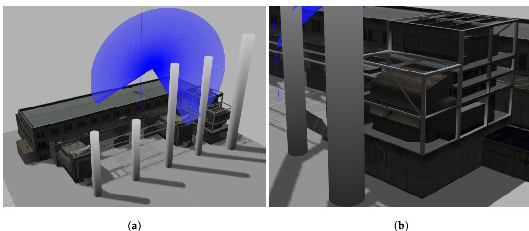
Figure 9. The model used to simulate the inspection scenario. (a) The factory to inspect with the UAV and a rendering of the sensor range. (b) A part of the structure impossible to cover safely.
