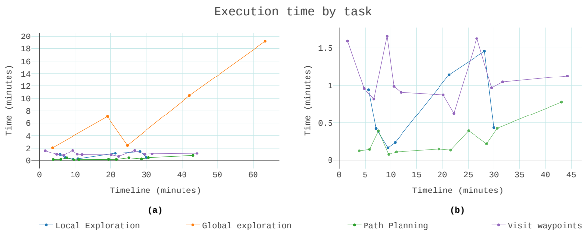
Figure 11. The execution time the mission manager spent in each task, in one run with a circular iterator. (a) All four tasks scaled together and (b) just local exploration, path planning, and visit waypoints.
