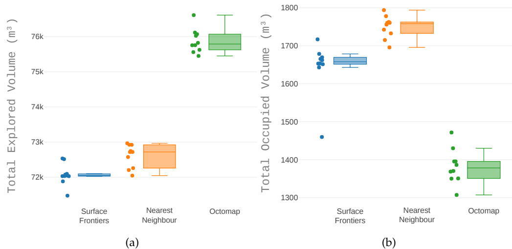
Figure 15. The volume explored at the end of the run for each of the analysed heuristics. Both (a) the total explored volume and (b) the volume of occupied space. The scales of the explored volume is one order of magnitude higher than the amount of occupied space, consequently (b) magnifies the difference of the outcome of each heuristic.
