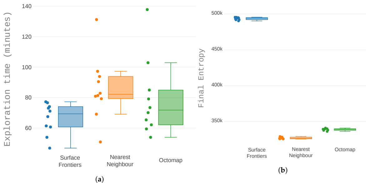
Figure 13. A comparison of the exploration with different heuristics: Nearest neighbour, octomap sector order, and closest surface frontier. Each heuristic was run 10 times. (a) Distribution of the time the system needs to complete the exploration task and (b) total entropy at the end of each run.
