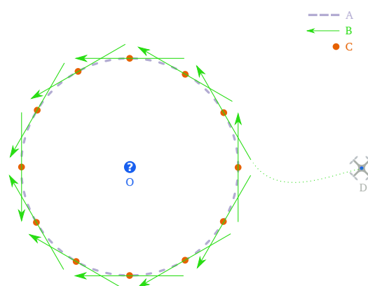
Figure 2. Circle (A) around the unknown location (O) with a radius equal to the sampling distance where different observation points (C) are shown. The green arrows represent the corresponding flyby manoeuvres for each observation point. The UAV is initially at position (D) and the final flyby manoeuvre is chosen to have the shortest path between this position and the start location of the flyby segment.
