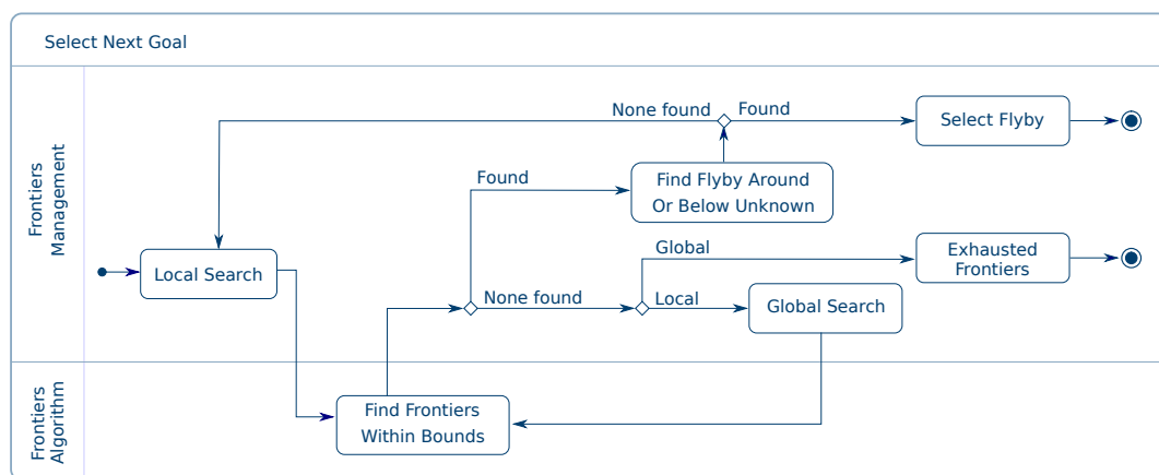
Figure 5. The activity diagram of the Frontier Manager node to find the next goal.
