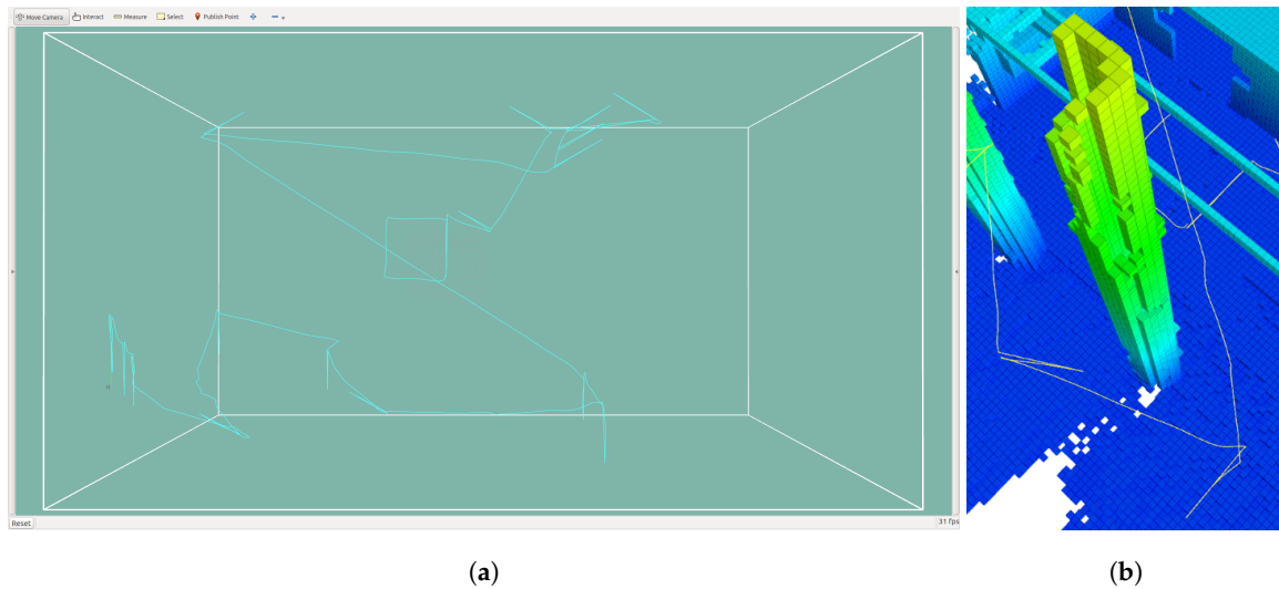
Figure 18. (a) Flight path with 507.3 m. (b) The flight plan adapts to the features of the structure.
