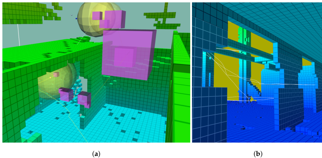
Figure 19. (a) Exploration transitions between indoors and outdoors seamlessly. The starting point is below. The target is represented by the unknown point above in dark blue. The yellow spheres represent the safety margin around each point. The required safe flight corridor in each segment has the same diameter. The purple cubes are the voxels containing each waypoint. The different sizes show the sparse quality of the octree. (b) The same detail viewed from inside the structure.
