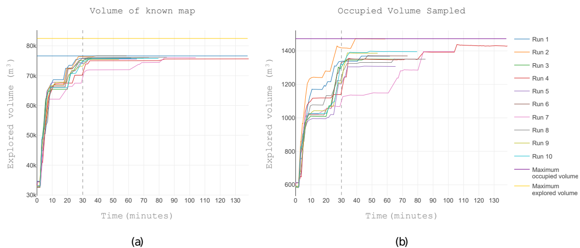
Figure 14. The volume explored in 10 runs. (a) Rate of exploration: Free and occupied are combined. (b) Coverage of the occupied volume.
