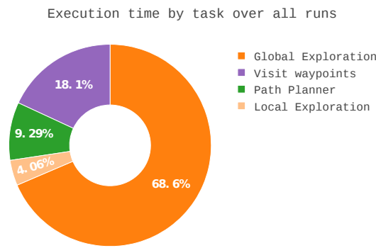
Figure 12. Distribution of the execution time of each task across ten runs.
