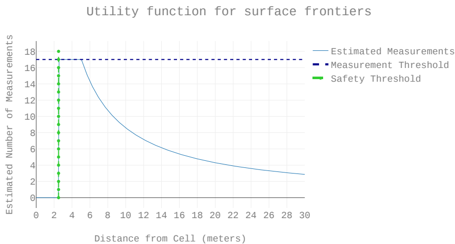
Figure 7. Equation (1) with h = 0.5 m, N = 1080 , d_s = 2.5 m, and t_m = 17 .
