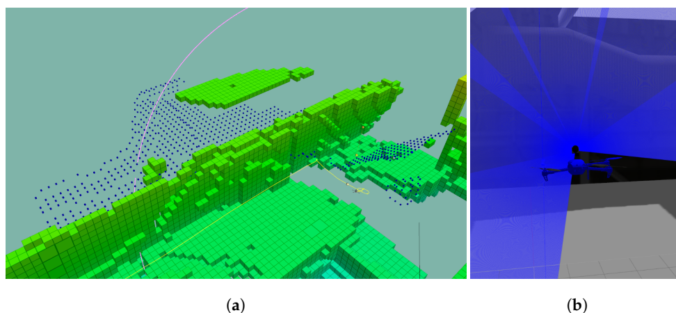
Figure 3. Neighbour generation, according to the sensor range. (a) The frontiers in blue could not be sampled as the only known space is above and the laser scanner has a blind spot below due to the 270^\circ scan angle. (b) The blue rays illustrate the range of the sensor. The scan angle is pointed upwards.
