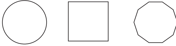
FIGURE 3. Some multi-rotationally symmetric planar convex bodies: the circle, the square and the regular decagon
