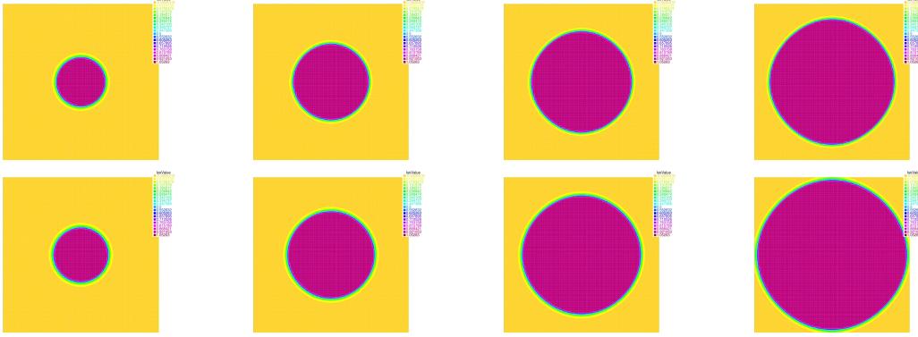
FIGURE 1. Evolution of the density at times t = 0.1, 0.2, 0.3, 0.4 for \alpha = 0.5 (top) and 1 (bottom).
