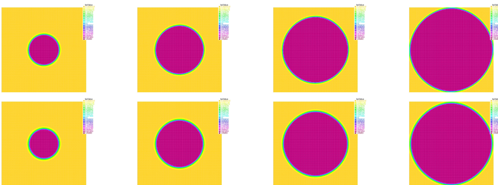
FIGURE 5. Comparison of the density at times t = 0.1, 0.2, 0.3, 0.4 for different k = 10 (top) and 1000 (bottom).
