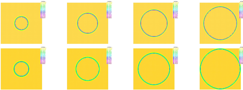
FIGURE 3. Evolution of the difference between the density and pressure at times t = 0.1, 0.2, 0.3, 0.4 for \alpha = 0.5 (top) and \alpha = 1 (bottom).
