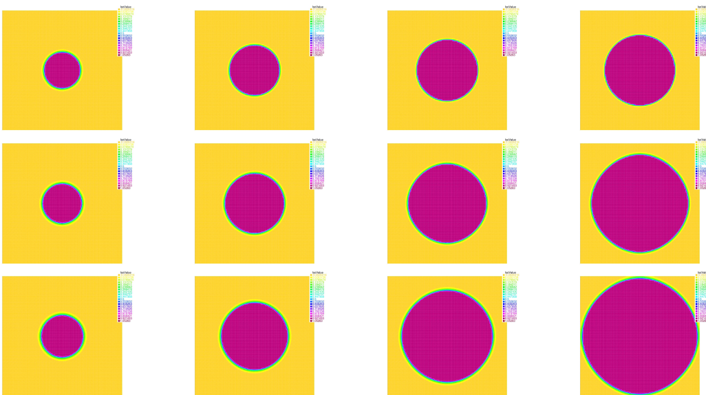
FIGURE 4. Comparison of the density at times t = 0.1, 0.2, 0.3, 0.4 for different \nu = 0 (top), 0.5 (middle), 1 (bottom).
