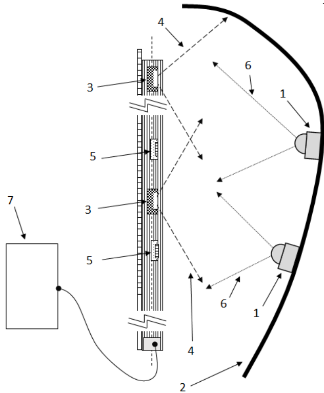
Figure 5: Application of proposed MOS for optical communication and control of devices (1) in cavities (2). LEDs (3) emit modulated light beams (4). Photodiodes (5) receive signals and data (6) from controlled devices (1) and send them to the control unit (7).
