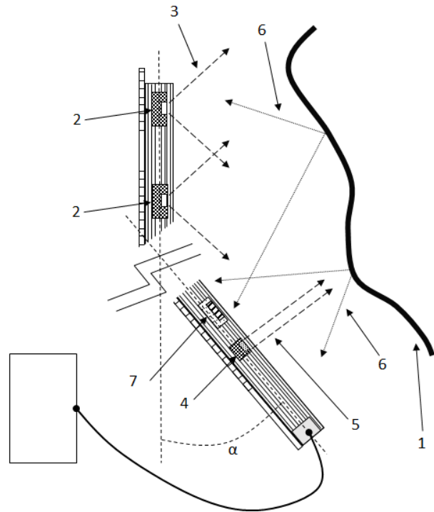
Figure 3: Application of proposed MOS for optical analysis of a surface (1). The optical strip is bended an angle \alpha . Each LED (2) emits a 90° cone of light (3). A laser diode (4) emits a collimated beam (5). Reflected light beams (6) are received by sensing photodiodes (7).
