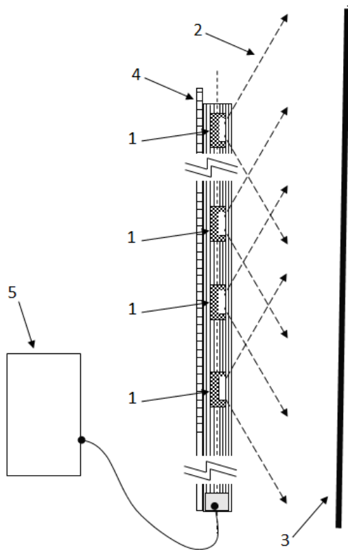
Figure 2: Application of proposed MOS as an illumination device. Each high-intensity LED (1) emits a 120° cone of light (2). For simplicity, the illuminated surface is shown as planar (3). The supporting metal layer (4) drains heat to dissipation elements in the control unit (5).
