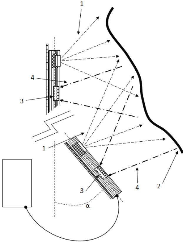
Figure 4: Application of proposed MOS for imaging inside cavities. The optical strip is bended an angle \alpha . Illumination or structured light beams (1) are projected onto the imaged surface (2). Imaging sensors (3) receive reflected beams (4).
