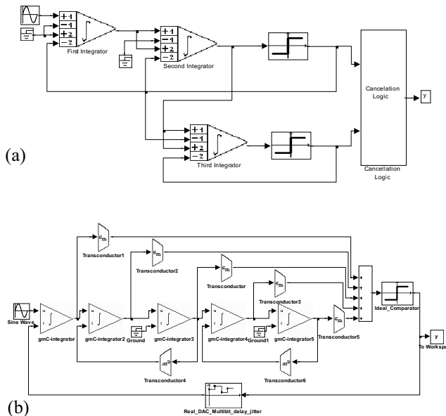
Fig. 6: Block diagrams of the (a) SC 2-1 sb \Sigma\Delta M and (b) CT 5th-order LP \Sigma\Delta M.
