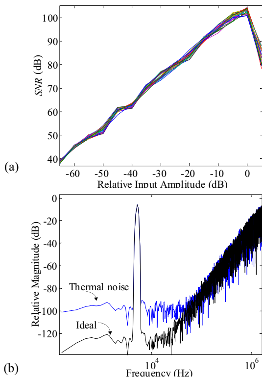
Fig. 7: Effect of (a) mismatch error and (b) thermal noise on SC 2-1 sb \Sigma\Delta M.
