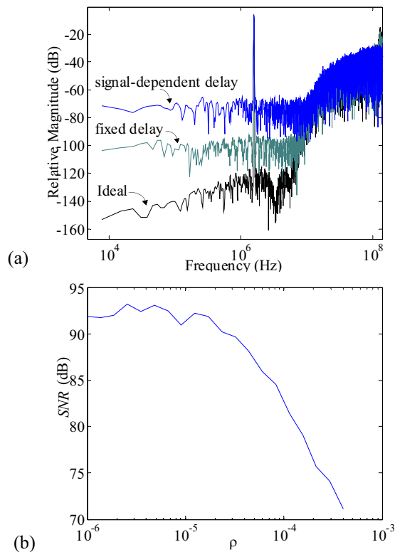
Fig. 8: Effect of (a) loop delay time and (b) clock jitter noise on CT 5th-LP \Sigma\Delta M.
